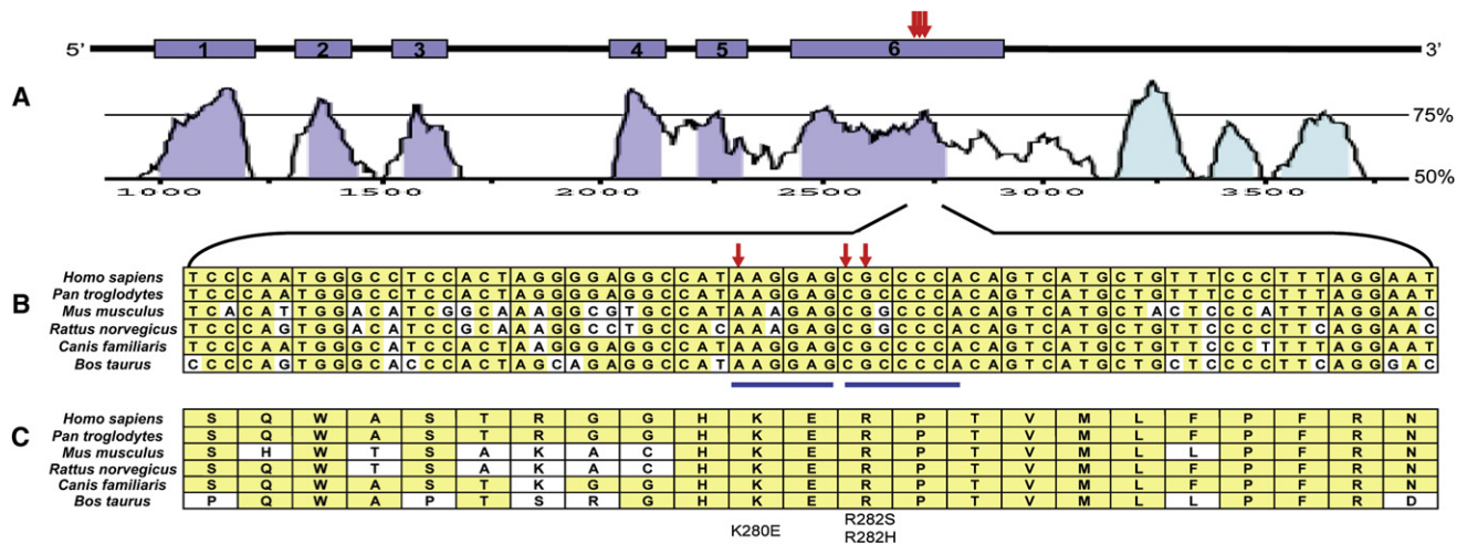
Figure 5. Genomic Structure and Evolutionary Conservation of TINF2
