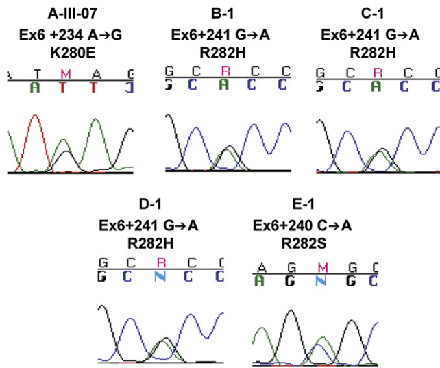
Figure 4. Representative Sequence Tracings of TINF2 Mutations
