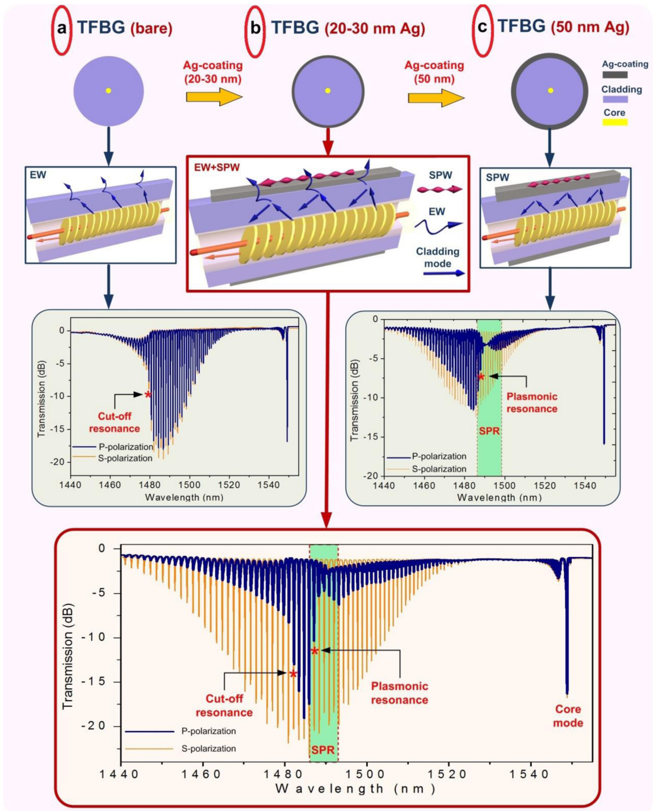
Fig. 4. Spectral characteristics of TFBG (20° tilted angle) versus different thickness of nanometric-coating: (a) bare TFBG without Ag-coating (a clear cut-off resonance at the boundary between guided modes (at longer wavelength side) and leaky modes (at shorter wavelength side)); (b) TFBG with 20–30 nm Ag-coating (hybrid “cut-off” and “plasmonic” resonances achieved simultaneously over a single TFBG); (c) TFBG with 50 nm Ag-coating (the normal thickness range for “plasmonic” excitation without leaky modes (at shorter wavelength side)). Note: red stars mark the corresponding position of “cut-off” and “plasmonic” resonances; P and S polarizations corresponds to two orthogonal polarizations in which SPR excitation over the P polarization; All above transmission spectra are measured from one TFBG in the same water solution (RI = 1.332). (For interpretation of the references to color in this figure legend, the reader is referred to the web version of this article.)
