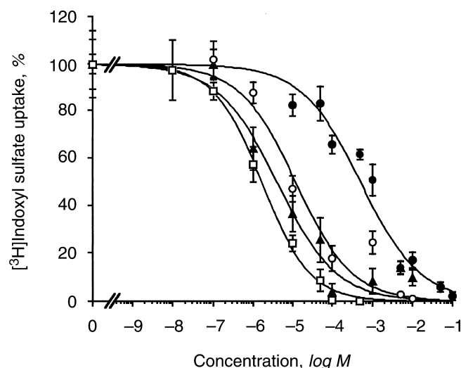
Fig. 4. Inhibition profile of rOAT3-mediated [ ^3 H]indoxyl sulfate uptake by probenecid (□), CMPF (▲), hippuric acid (○), and indole acetic acid (●). The values are expressed as a percentage of [ ^3 H]indoxyl sulfate uptake in rOAT3-expressing oocytes at one hour in the absence of inhibitor (mean \pm SEM; N = 8 to 10).
