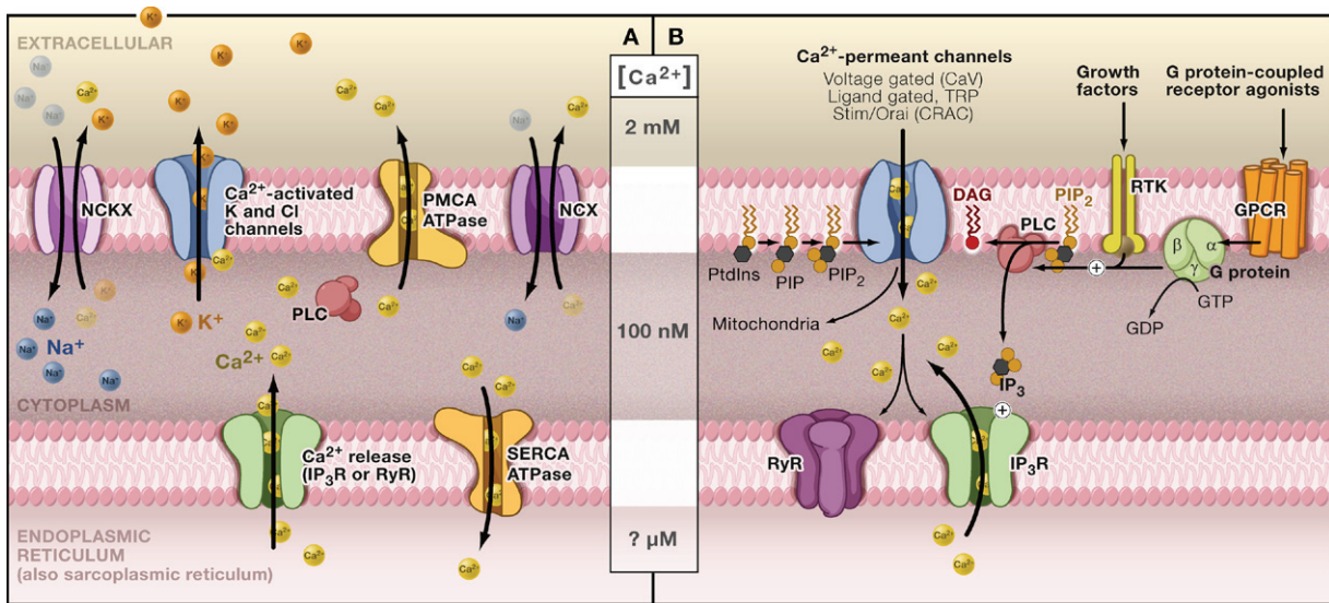
Figure 3. Maintaining and Using \text{Ca}^{2+} Gradients for Signaling
