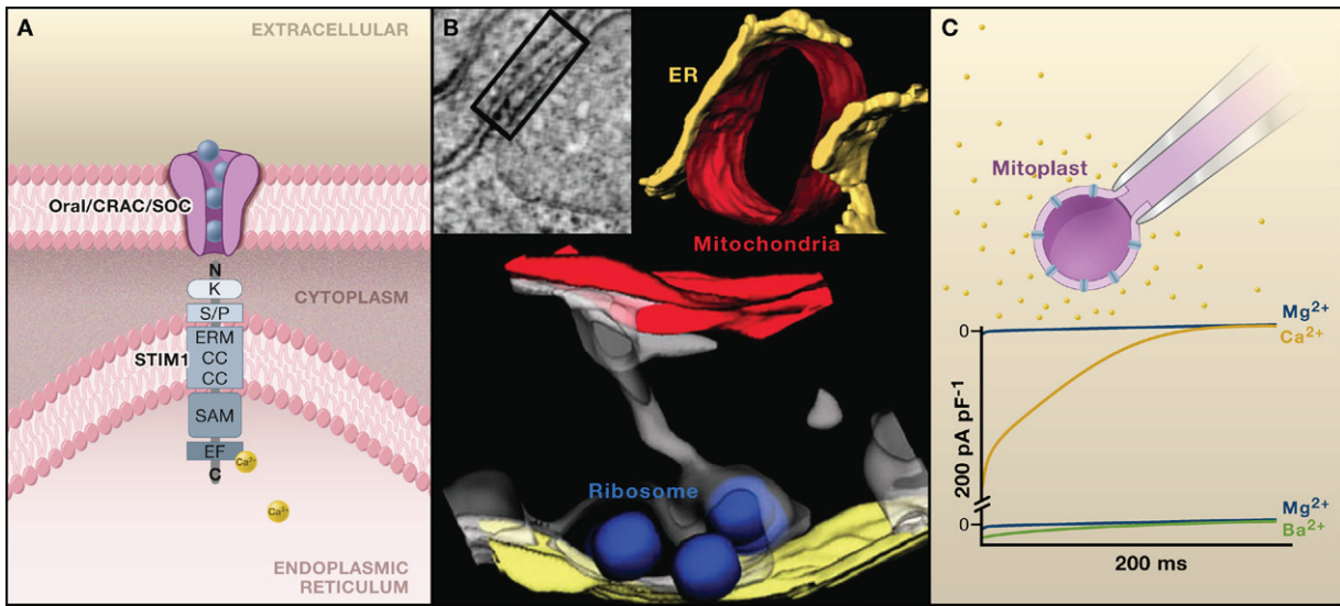
Figure 4. Emerging \text{Ca}^{2+} Pathways
