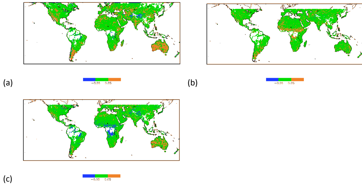
Figure S7 Differences in precipitation products in terms of their annual sum of positive Pearson correlation coefficients between high frequency soil moisture fluctuations and precipitation. (a) CMORPH-PERSIANN, (b) CMORPH-TRMM, and (c) TRMM-PERSIANN. The soil moisture data were taken from ascending (1330LT) overpasses of AMSR-E.
