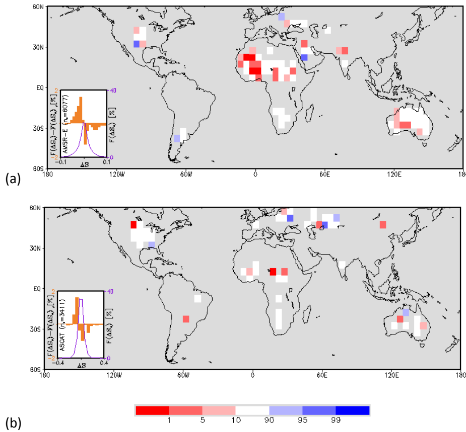
Figure S10 Preference for afternoon precipitation over soil moisture anomalies using coarse resolution data. As for Figure S5 except that the analysis was based on datasets with resolution of 1.0°.
