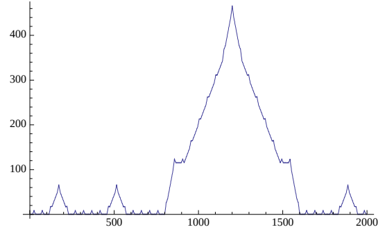
Figure 6: The 7-adic valuation of T(n)
