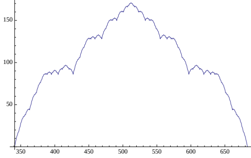
Figure 3: The 2-adic valuation of T(n) between minima
