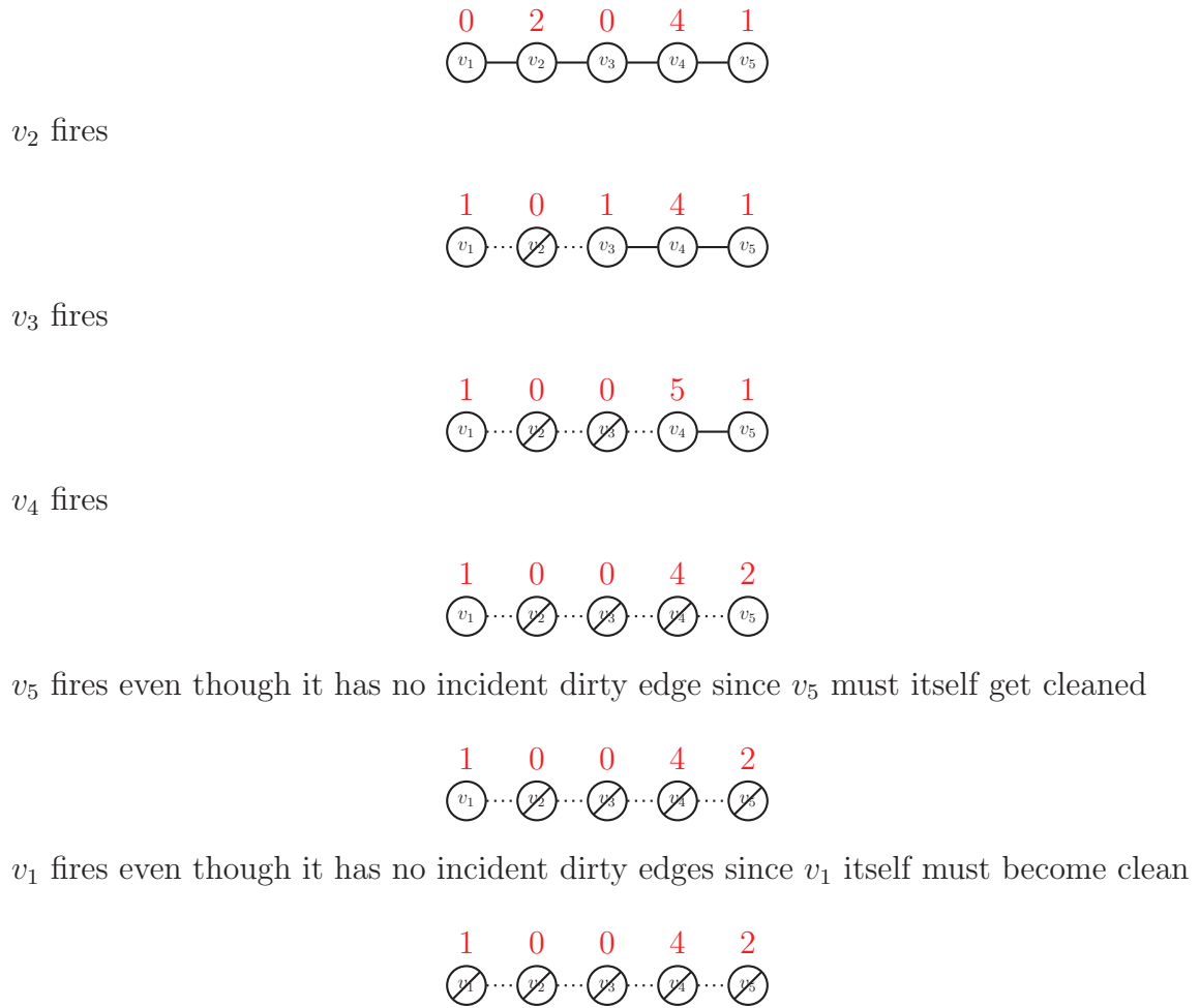
Figure 2.2: Sequential Brushing example on P_5 which will return no dirty vertices.
