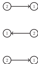
Figure 5.3: Period of P_2^{2-1}
