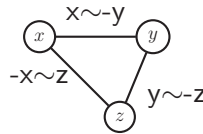
Figure 5.14: Triangle created by adding a third edge labelled -x \sim z
