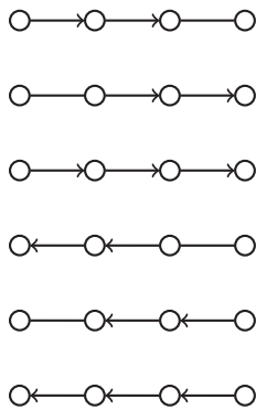
Figure 3.11: List of orientations which cannot exist as suborientations within a p_2 -orientation
