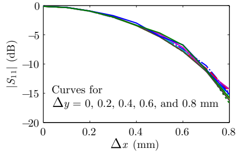
Fig. 3 Simulated depth of notch versus \Delta x , at the fix frequency f = 4.253 GHz, for different values of \Delta y from 0 mm to 0.8 mm in steps of 0.2 mm. Due to the symmetry of the proposed sensor, an identical plot also describes dependency to displacement in x direction for |S_{22}| versus \Delta y .
