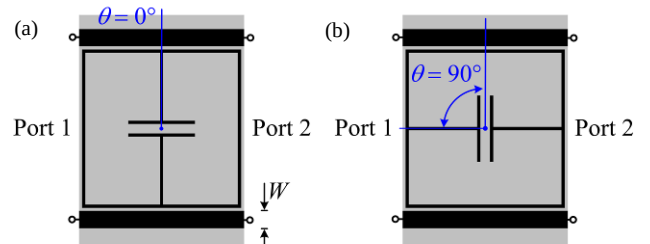
Fig. 2 Parallel microstrip lines loaded with an ELC resonator for the two extreme cases of angular orientation; (a) \theta = 0^\circ and (b) \theta = 90^\circ .
