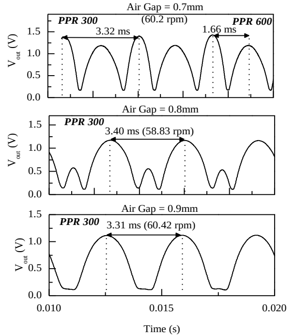
Fig. 18. Envelope of the modulated carrier signal for different air gaps, corresponding to the rotor with a single chain of SRRs. For the smaller air gap, the amplitude of the pulses is similar, and the angular velocity can be obtained from the time distance between adjacent pulses, or between higher amplitude pulses, as indicated.
