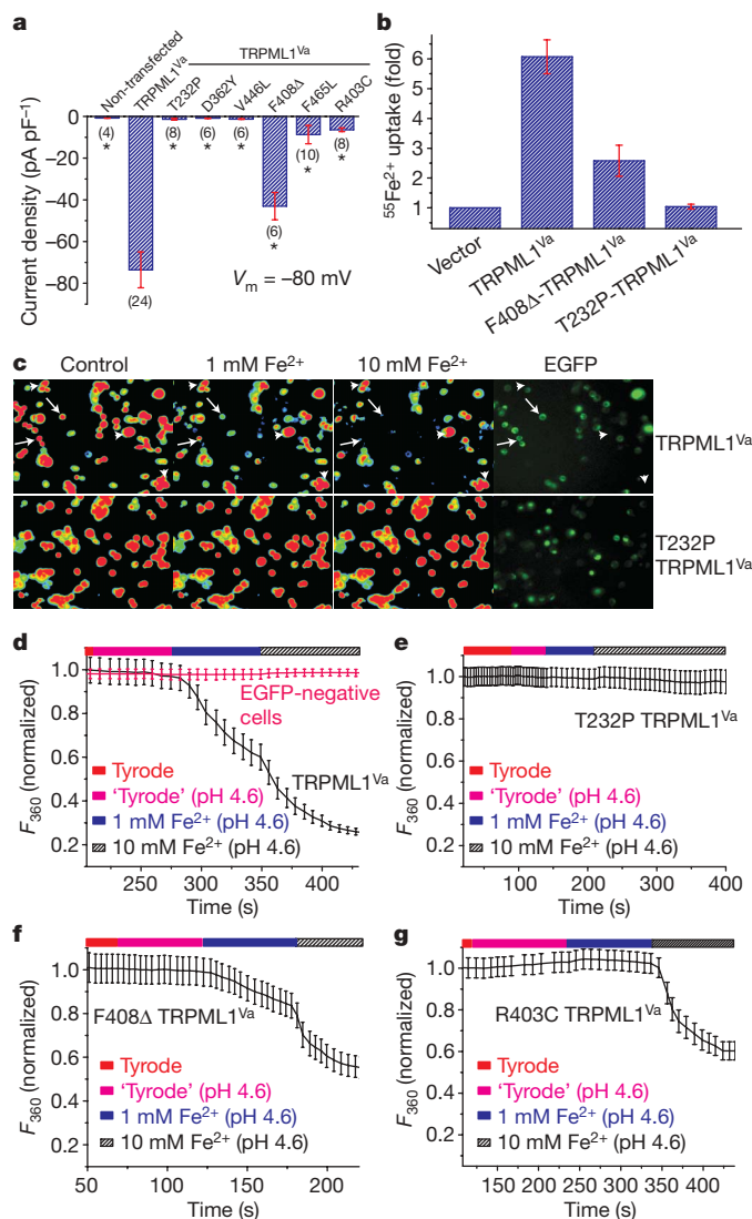
Figure 2 | Fe 2+ permeability of the TRPML1 channel is impaired by ML4 mutations. a , Current densities (mean \pm s.e.m., n = 4-10 ) of I_{\text{Fe}} ( 30 mM \text{Fe}^{2+} , pH 4.6 ) for TRPML1 Va and ML4 mutant TRPML1 Va channels. Asterisk indicates statistical difference ( P < 0.01 ) compared to TRPML1 Va . b , ^{55}\text{Fe}^{2+} uptake (normalized) in HEK293T cells transfected with vector control, with TRPML1 Va , with F408 \Delta -TRPML1 Va and with T232P-TRPML1 Va constructs. Error bars indicate the standard deviation on the basis of two independent triplicate experiments. c , [\text{Fe}^{2+}]_o -dependent quenching of Fura-2 fluorescence in TRPML1 Va -transfected cells (arrows), but not in non-transfected control cells (arrowheads) or T232P-TRPML1 Va -transfected cells (bottom row). The fluorescence intensity was measured at an excitation wavelength of 360 nm ( F_{360} ). The original magnification used for all micrographs was \times 200 . d , Average normalized responses of EGFP-positive TRPML1 Va -transfected cells (typically n = 20-40 cells) to 1 or 10 mM \text{Fe}^{2+} (pH 4.6 ). e , No significant quenching was seen in T232P-TRPML1 Va -transfected cells. f , Slightly less quenching was observed for the F408 \Delta -TRPML1 Va -expressing cells. g , A small but significant quenching reaction was detected (with 10 mM \text{Fe}^{2+} ) in R403C-TRPML1 Va -expressing cells.
