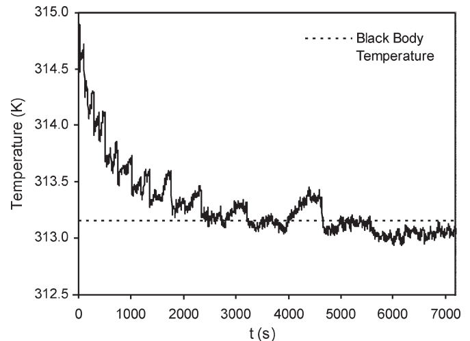
Fig. 3. Changes of the radiometric temperature measured by the camera after power-on over the course of 2 h.
