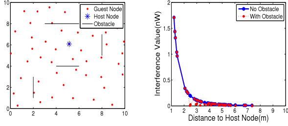
(a) The Deployment of the Sensor Nodes (b) The Interference to the Host Node
