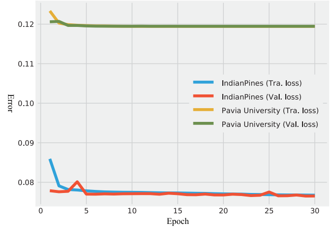
Fig. 4. Learning curves for the initial fully Conv-Deconv network on the Indian Pine data set and the Pavia University data set. Although the network starts greatly reducing errors on both the training and validation samples during the first few epochs, it rapidly converges to a fairly high value, which means the learning of the network is significantly slowed down and eventually gets stuck into a local minimum. This indicates that such a network architecture is not easy to optimize.
