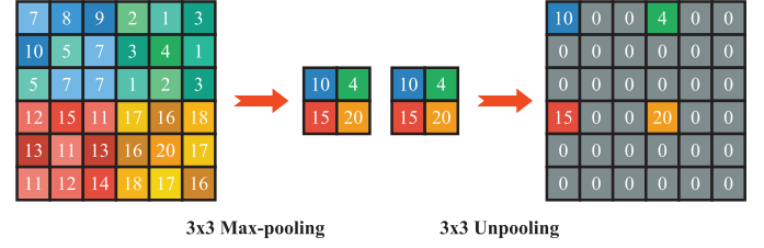
Fig. 3. Illustration of (Left) max pooling and (Right) unpooling as used in the fully Conv-Deconv network described in Section III-A.
