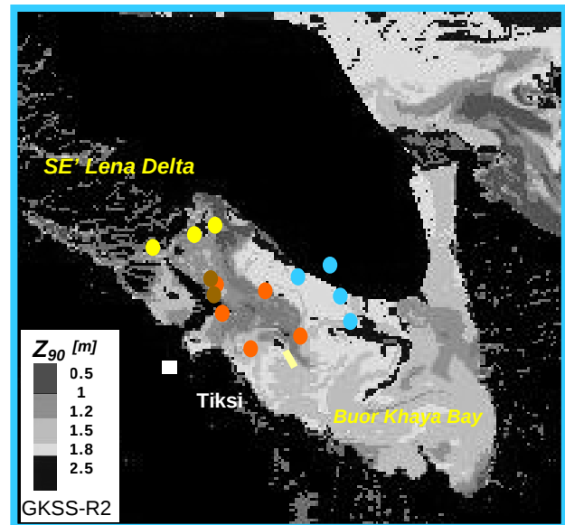
Figure 2. MERIS RR, 2008-13-08, 11:38 local time, MERIS C2R processor: 'attenuation depth, 'Z90'', (thin clouds manually masked in black). Lena08-expedition stations: near-shore waters of Ice-Complex (brown), on-shore (orange), offshore (blue), estuarine waters (yellow).
