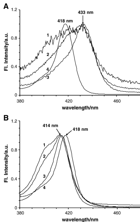
Fig. 1. Normalized fluorescence excitation spectra of PPhe ( \lambda_{\text{em}}=640 nm) in aqueous solution and in the presence of DMPC vesicles at (A) pH=3 and at (B) pH=7: 1 — [PPhe]=1 \mu M and T=32 °C; 2 — [PPhe]=0.1 \mu M and T=32 °C; 3 — [PPhe]=0.1 \mu M and T=62 °C; 4 — [PPhe]=0.1 \mu M, [DMPC]=0.25 mM and T=32 °C.
