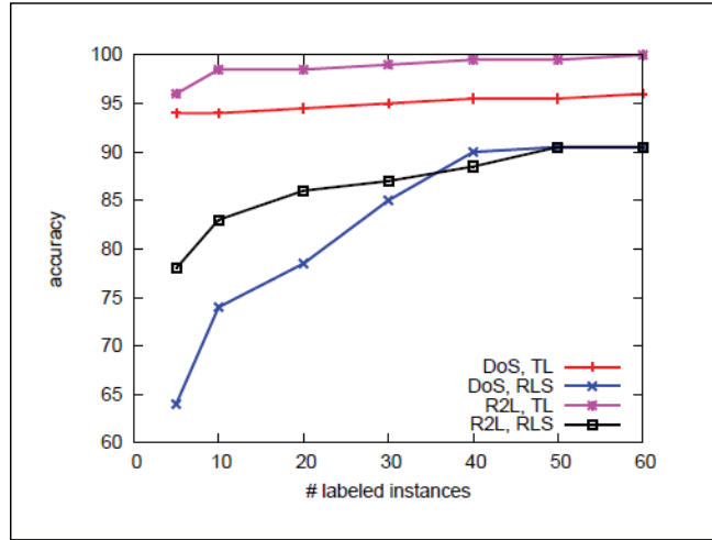
Fig. 1.2. Performance of Algorithm TL with limited labeled data. The plot shows how classifier accuracy (vertical axis) varies with the number of available labeled target instances (horizontal axis) for four tasks: distinguish N and DoS using RLS classifier, distinguish N and DoS using Algorithm TL, distinguish N and R2L using RLS classifier, and distinguish N and R2L using Algorithm TL.
