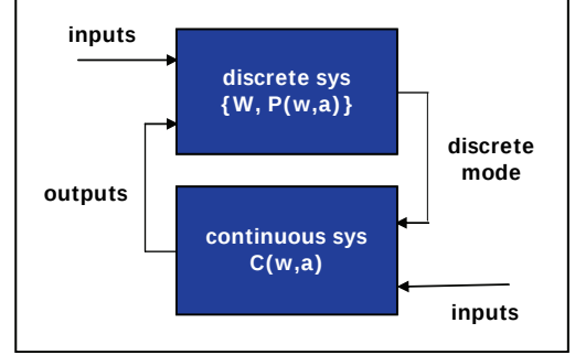
Figure 3. Schematic of basic HM-HDS feedback structure. The discrete and continuous systems in this framework model the selection of “active” classifier w_a and the resulting attack-defend dynamics, respectively.
