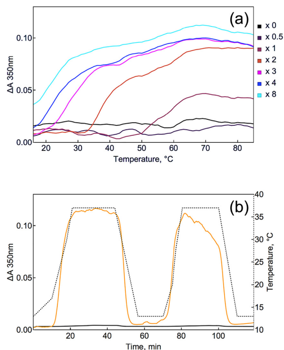
Fig. 1. (a) Temperature dependence of 30 \mu M tau samples turbidity in the absence of \text{ZnCl}_2 (black curve) and in the presence of 0.5-, 1-, 2-, 3-, 4- and 8-fold molar excess of \text{ZnCl}_2 (see color legend on the right) in 50 mM Tris buffer and 1 mM TCEP at pH 7.5 obtained using Prometheus NT.Plex instrument. (b) Reversible aggregation of tau (30 \mu M) followed by turbidimetry in the presence of 4-fold molar excess of \text{ZnCl}_2 (yellow curve); control tau sample in the absence of zinc (black curve); variation of temperature during experiment (black dotted line). Measurements were carried out using PerkinElmer spectrophotometer Lambda 800.
