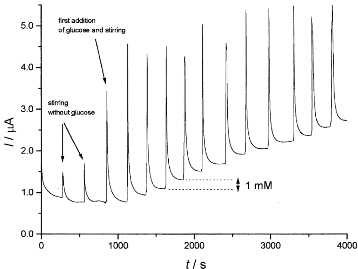
Figure 5: Amperometric response of the (PEG-GOD/PEDT) electrode versus glucose concentration (between 0 and 10 mM). E=0.3 V vs. Ag / AgCl. The medium is deaerated 0.05 M phosphate buffer (pH 6) containing 0.05 M KCl+3×10 -4 M ferrocenemethanol. Successive additions (corresponding to 1 mM glucose) were injected at room temperature, under stirring for 5 s. Film thickness: 20 nm.
