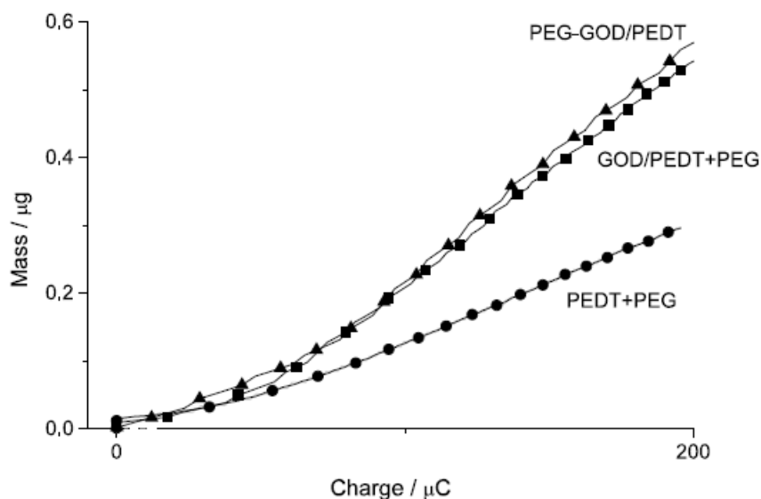
Figure 4: Data from ECQM: electrode mass versus charge during the potentiostatic electrosynthesis of (a) (PEDT+PEG) film (•), (b) (GOD/PEDT+PEG) film (◼) and (c) (PEG-GOD/PEDT) film (◴). Quartz surface: 0.2 cm 2 . Films were grown until a charge of 200 μC was reached, in 0.05 M phosphate buffer (pH 6) containing 0.05 M KCl+10 -2 M EDT+10 -4 M PEG (a), 10 -4 M PEG+1000 IU ml -1 GOD (b) or 10 -4 M PEG+1000 IU ml -1 PEG-GOD (c).
