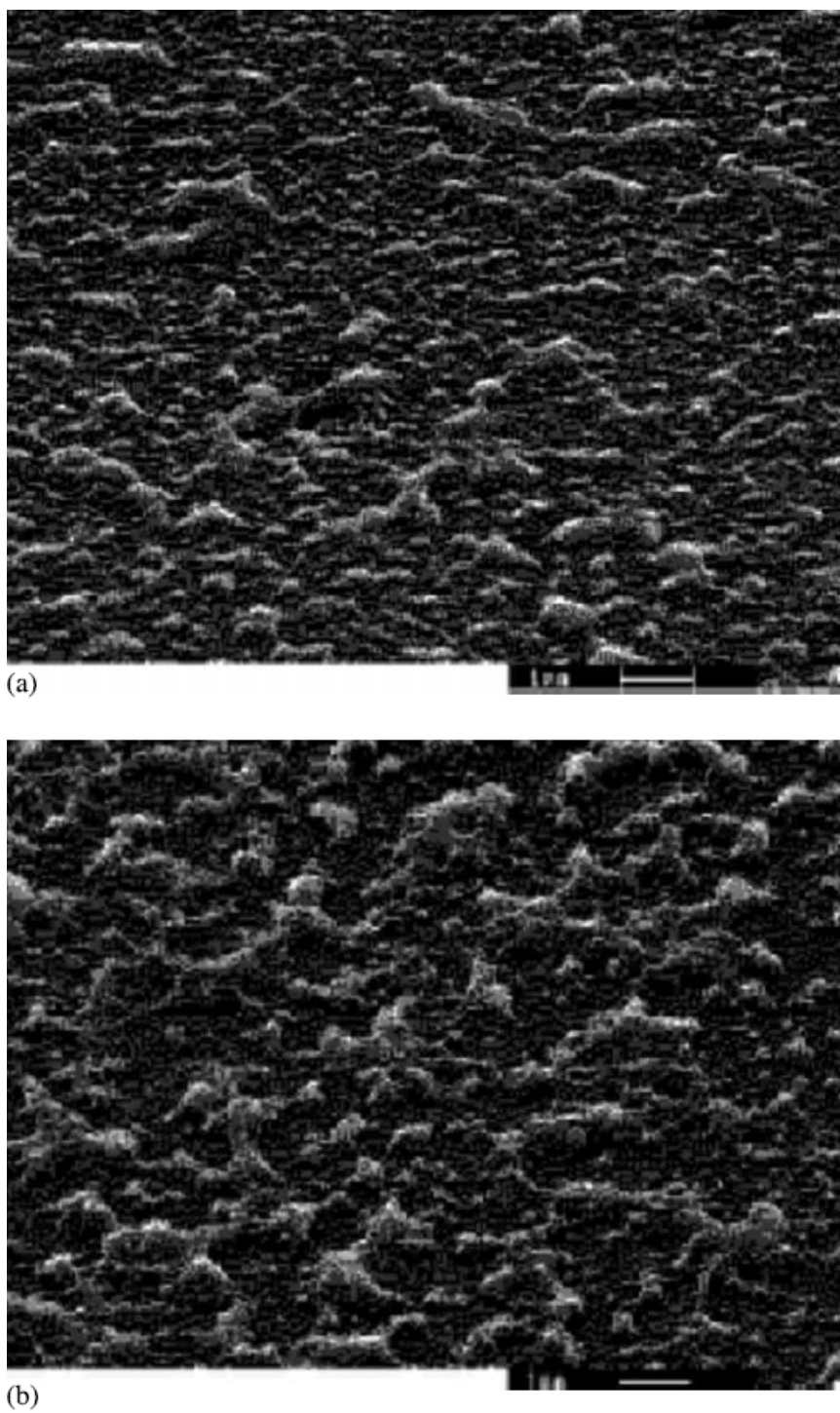
Figure 2: SEM pictures of films electrodeposited on a GC electrode at constant potential +1.1 V for 10 s: (a) (PEDT+PEG) and (b) (PEG-GOD/PEDT).
