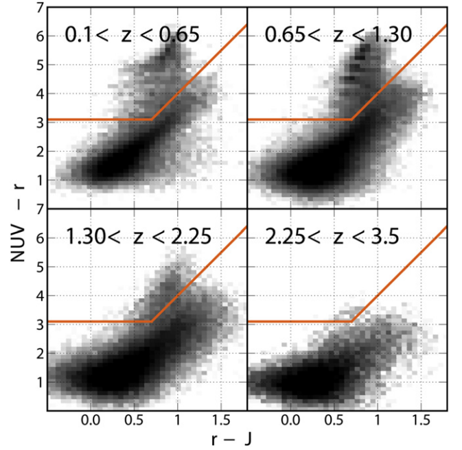
Figure 16. NUV - r/r - J galaxy distributions. Quiescent galaxies lie in the top-left corner. The objects fainter than limiting magnitudes are not used.
