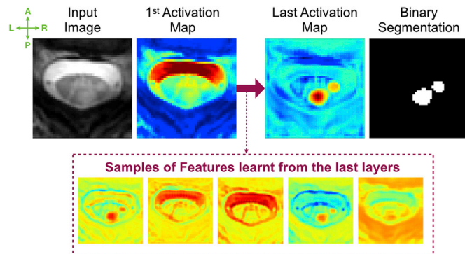
Fig. 7. Visualisation of feature map instances, learnt by different layers of the CNN 2-Lesion , applied to an input image (left) leading to a binary segmentation (right). The normalised values represent the responses to filters learnt during the training step, with a colormap from blues (weak filter match) to reds (strong filter match).
