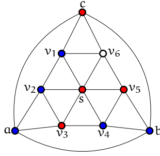
Figure 3.4.: A plane graph that does not admit a guard coloring. Assume that we want to find a guard coloring in red and blue. Face (a, b, c) must not be monochromatic, so without loss of generality we choose a and b to be blue while c is red. Then either v_1 or v_6 needs to be blue. The graph is symmetric, so we choose v_1 to be blue. Then v_2 must be blue as well to have a monochromatic edge incident to face (a, v_2, v_1, c) . In the next step, we color v_3 and s red, because otherwise we would get monochromatic faces. For the same reason v_4 then becomes blue and v_5 becomes red. This leaves only v_6 uncolored. It cannot be red, as triangle (s, v_5, v_6) would become monochromatic, and it cannot be blue, as triangle (c, v_6, v_5, b) would have no monochromatic edge.
