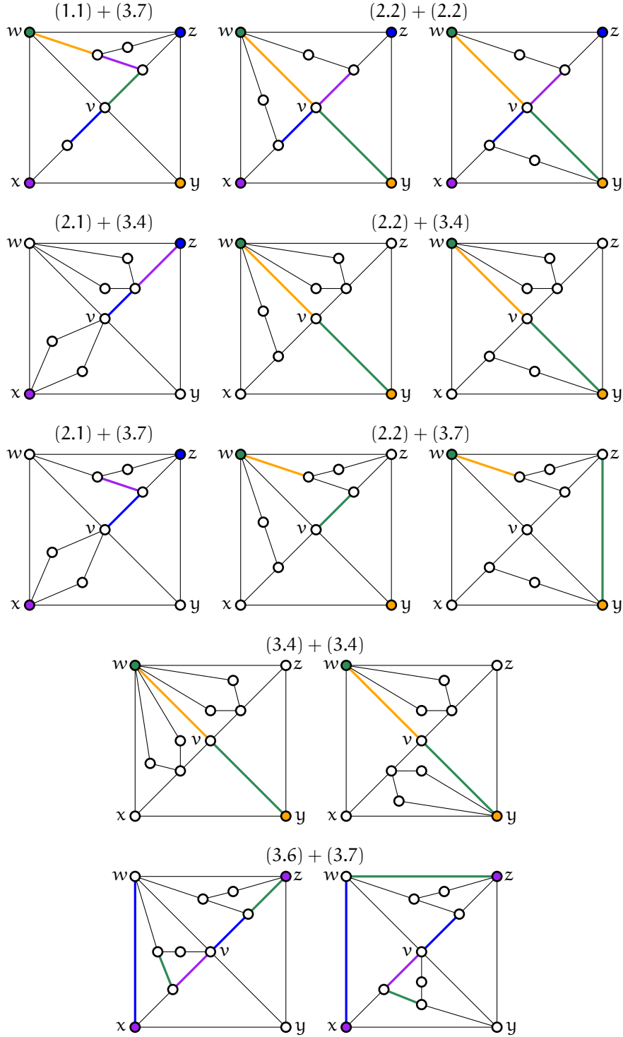
Figure B.4.: Special cases from the proof of Lemma 5.6 that need to be considered one by one.
