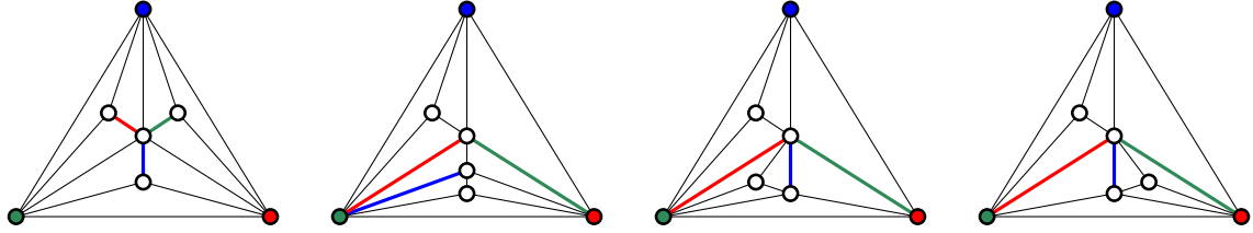
Figure 4.5.: The four possible stacked triangulations with seven vertices that are not formed from a stacked triangulation with six vertices and an additional outer vertex. The colors encode how to form an edge guard set using one additional edge: If for example the green outer vertex is a vertex guard, the thick green edge can be used to guard the remaining faces.
