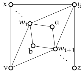
Figure B.6.: Vertices w_i and w_{i+1} share two neighbors a and b of a deeper level. Then S(w_i) \cup S(w_{i+1}) = \{w_i, w_{i+1}, a, b\} and all four of them can be removed. Edge vw_i extends any edge guard set of the obtained smaller graph to an edge guard set for the original graph.
