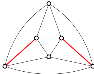
Figure 3.1.: The octahedron graph with two edge guards (shown in red). No single edge guards all of its eight faces.
