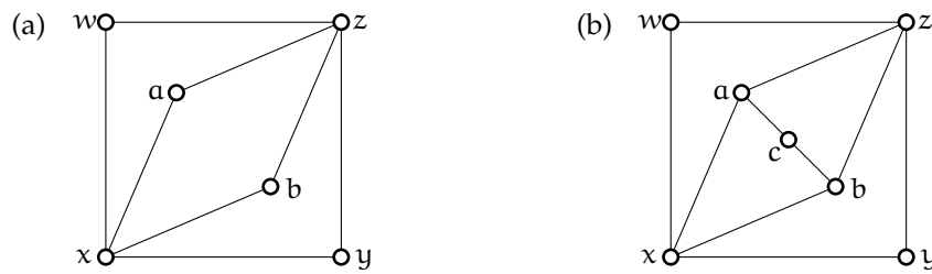
Figure B.1.: (a) The face f subdivided by vertices a and b . Any edge guard set contains at least one vertex from \{x, z\} . (b) The face f subdivided by vertices a, b and c . Any edge guard set contains either both \{x, z\} or an edge with both endpoints in \{a, b, c, x, z\} .
