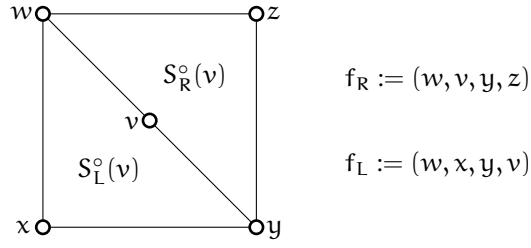
Figure B.2.: Vertex v lies inside quadrangle (w, x, y, z) and subdivides it into two faces f_L := (w, x, y, v) and f_R := (w, v, y, z) . Both of them can be further subdivided by vertices in S^o(v) where S_L^o(v) is inside f_L and S_R^o(v) is inside f_R .
