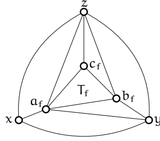
Figure 4.2.: Face f of S with boundary vertices \partial f = \{x, y, z\} gets subdivided by the three vertices a_f, b_f and c_f , which form a face in G .
