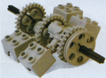
8860 Car chassis
