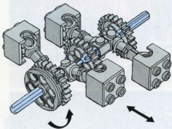
8860 Car chassis
