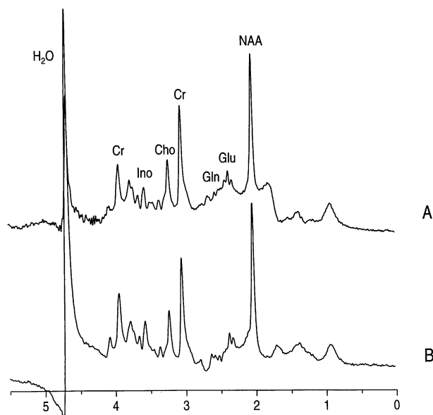
Figure 4. A: Spectrum acquired from a human brain using the MEGA-STEAM sequence shown in Fig. 2A ( TE = 34 ms, TM = 10 ms, TR = 3 s, voxel size = 27 mL, NEX = 64, 1 Hz line broadening, total acquisition time = 3.2 min). The carrier frequency of the selective pulses was placed on the water resonance. Note that excellent suppression of the water resonance was achieved without distorting the phase of resonances outside the selective pulse bandwidth. B: For comparison, a 3,1-DRYSTEAM spectrum was acquired from the same subject and location using a TR = 3 s, TE = 34 ms and TM = 33 ms (NEX = 64), and using identical processing. Note that the water peak of this spectrum extends well above the highest peak of the MEGA spectrum shown in A.
