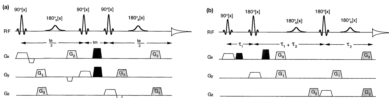
Figure 2. The sequence element MEGA as implemented in STEAM is shown in A. Excitation pulses and gradient waveforms for the PRESS sequence incorporating MEGA are illustrated in B. Gradients G_1 , G_2 and G_3 are used for MEGA implementation in both sequences. For suppression of the water signal only, a single-banded frequency selective pulse is used
