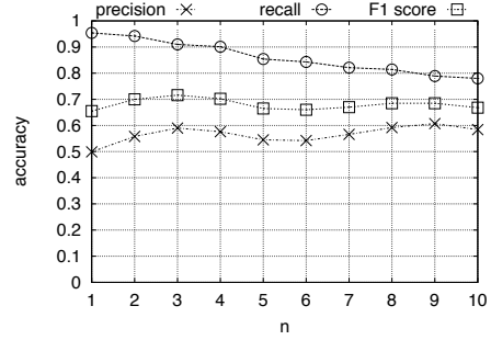
(b) Random forests and naive aggregation (used in SmartFABER)
