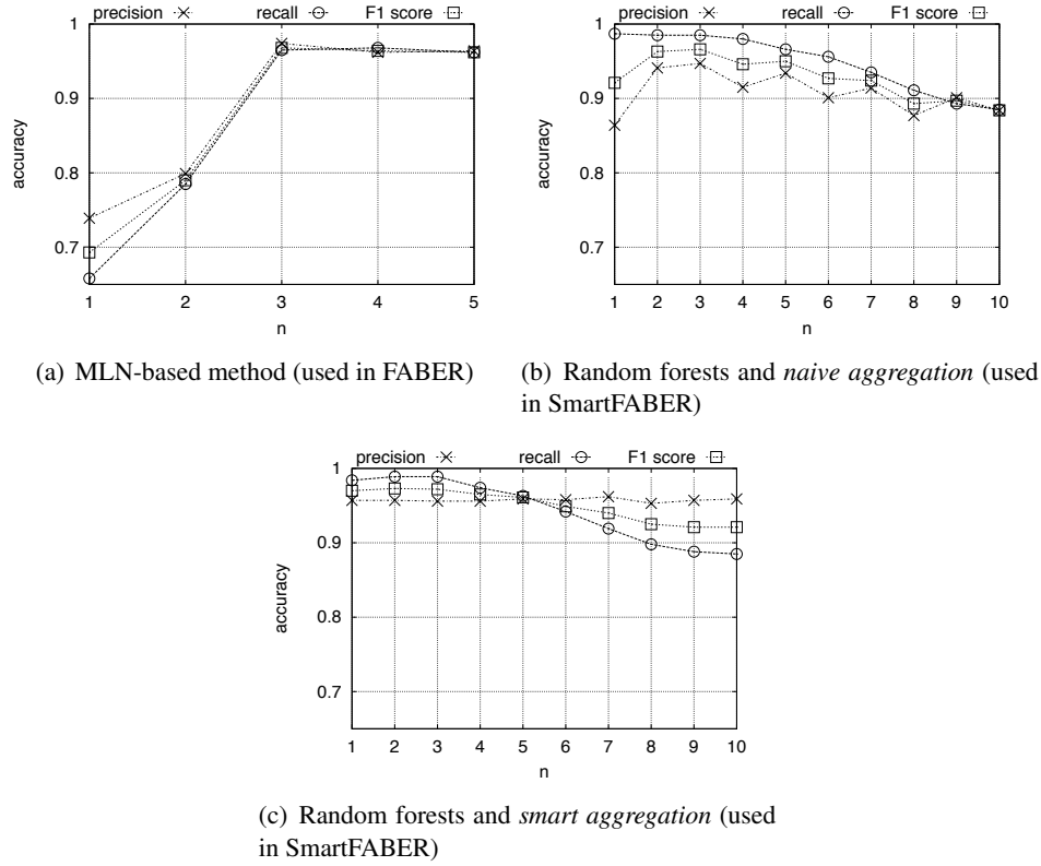
Figure 7: Smart home lab dataset. Accuracy of activity boundary detection; n is the length of the considered temporal sequence of sensor events
