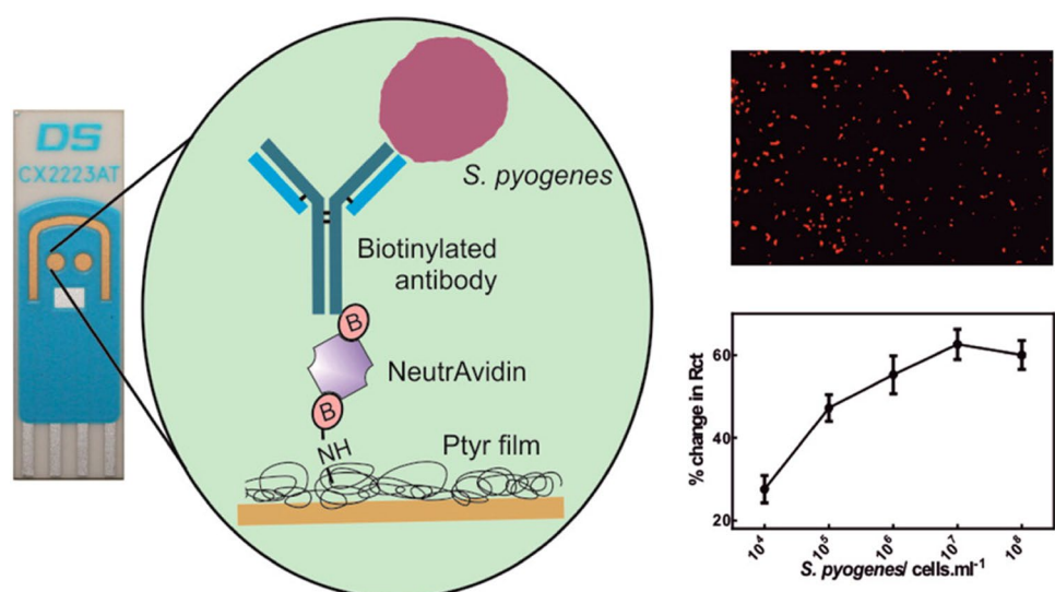
Fig. 8 On the left, there is the general scheme of immunosensor against Streptococcus pyogenes construction layer-by layer over a DropSens gold SPE (CX2223AT). On the top right, a fluorescence imaging of bound S. pyogenes on the sensor surface. On the bottom right, there is a % change in impedance plot upon the addition of different bacteria concentration, from 10^4 to 10^8 cells/mL. Reproduced from [41], with permission of ACS
