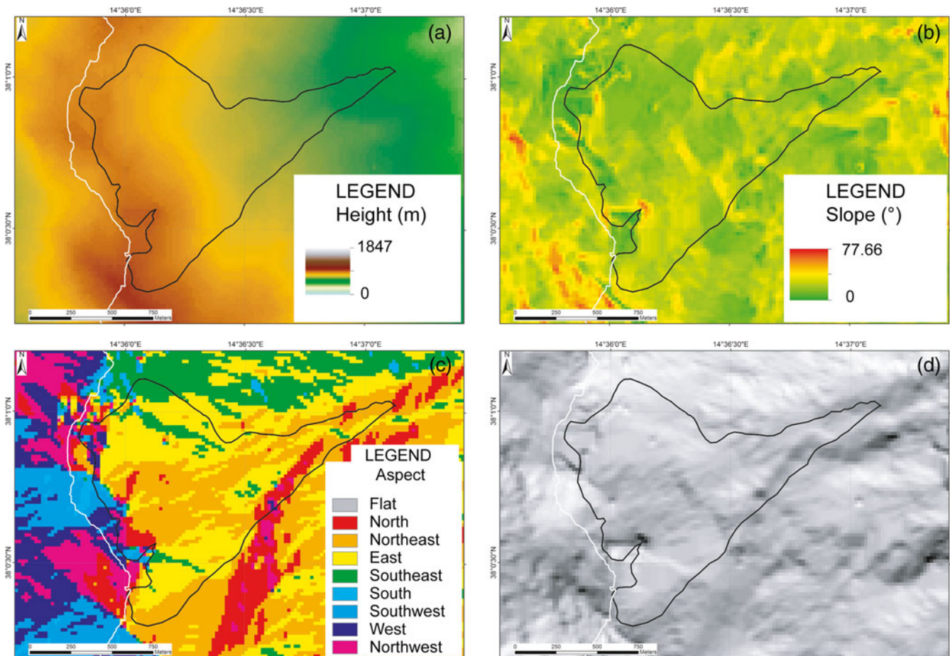
Fig. 2 Example of the 20-m resolution DEM-derived products for the area of San Fratello. a DEM, b slope, c aspect, and d hillshade. The white line is the watershed divide; the black line corresponds to the 2010 landslide boundary
