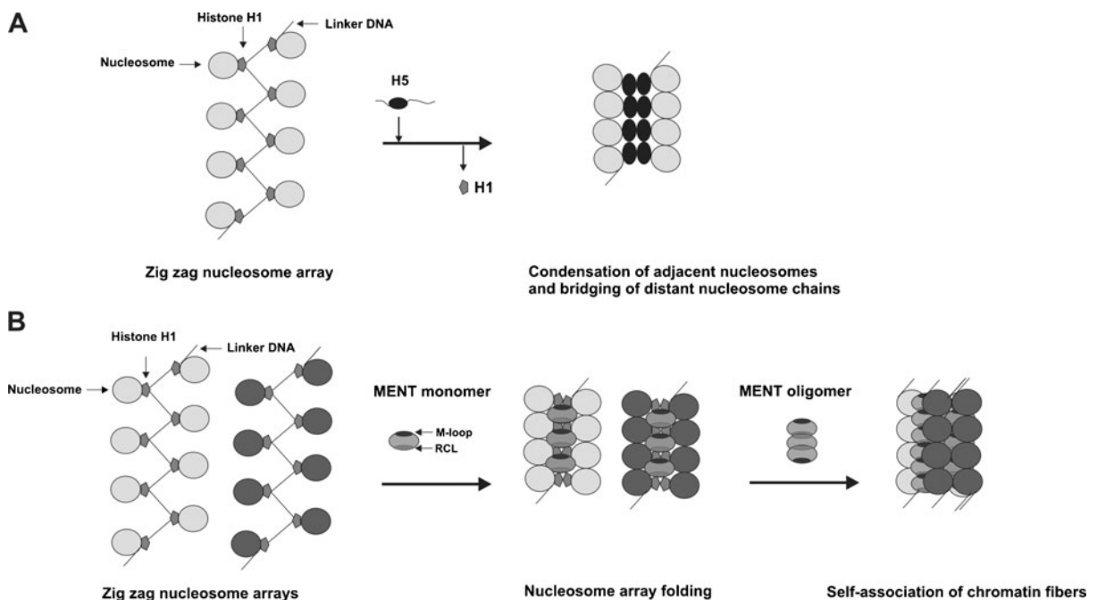
Fig. 2 Models for the formation of compacted chromatin fibers. a A formation of dense chromatin structure by histone H5-mediated association of adjacent nucleosomes and bridging of distant nucleosome chains. A side-by-side self-association of compacted neighboring poly-nucleosome arrays
