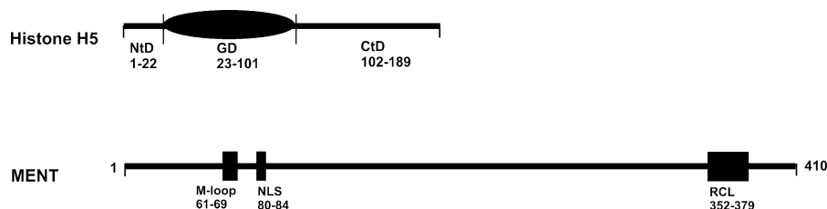
Fig. 1 A domain structure for histone H5 and MENT molecules. While the histone H5 is composed of a globular domain (GD, residues 23–101) flanked by an N-terminal domain (NtD, residues 1–22) and C-terminal domain (CtD,
