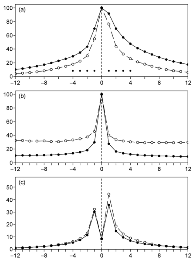
Figure 2 The ratio (units: %) of composed rainfall (a) frequency and (b) intensity before and after the rainfall peak to that at the peak time (time zero) averaged in 102°–122°E, 20°–40°N in the warm season (May–October) during 1961–2006. The dotted solid lines (dashed lines with circles) are for the intense rainfall (weak rainfall). The differences of frequency before and after the peak time of intense rainfall in (a) is significant at the 10% confidence level according to Student's t -test and the time when rainfall accounts for more than 10% of the differences are marked by black dots at the bottom of (a). (c) Same as in (a), but for the percentages of rainfall with intensity greater than 30% of that at the peak time to the total frequency at each time (except time zero); the percentage at time zero represents the rainfall with intensity greater than 30% of that at the peak time to total rainfall at both 1 h before and after the peak time.
