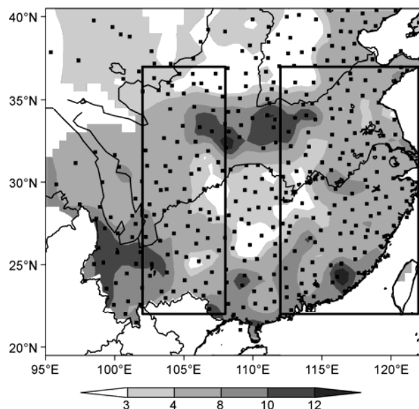
Figure 1 Locations of 392 rain gauge stations and the e-folding decay rainfall intensity (shaded, units: mm h -1 ). Two subregions, the western region (102°–108°E, 22°–37°N) and eastern region (112°–122°E, 22°–37°N) are outlined for regional average.
