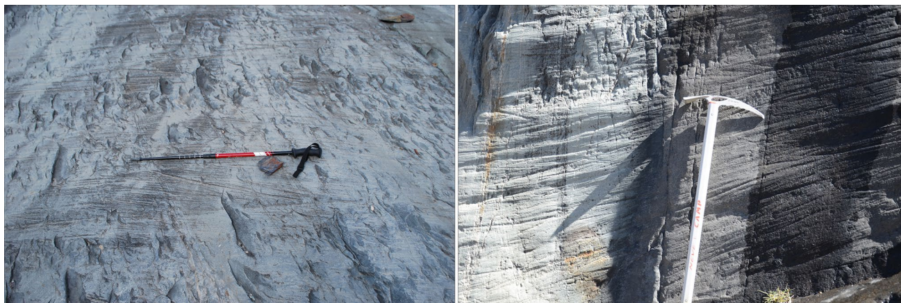
Fig. 6 Striations observed on the rocks during fieldwork
