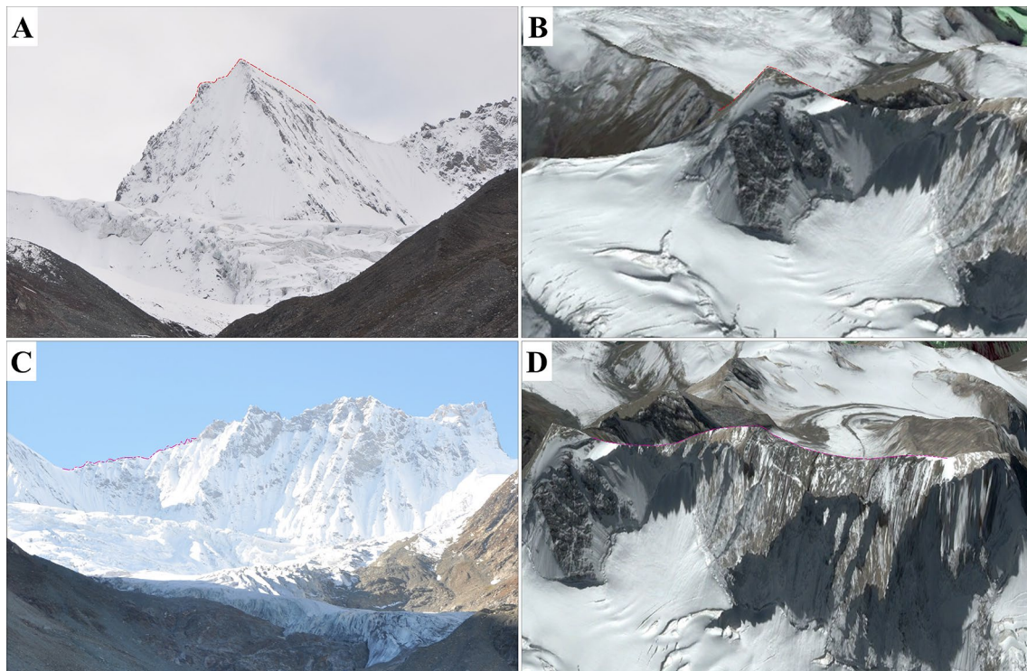
Fig. 4 a Field photograph of the horn; b Horn on the satellite image; c Field photograph of the serrate arête and d serrate arête seen on the satellite image
