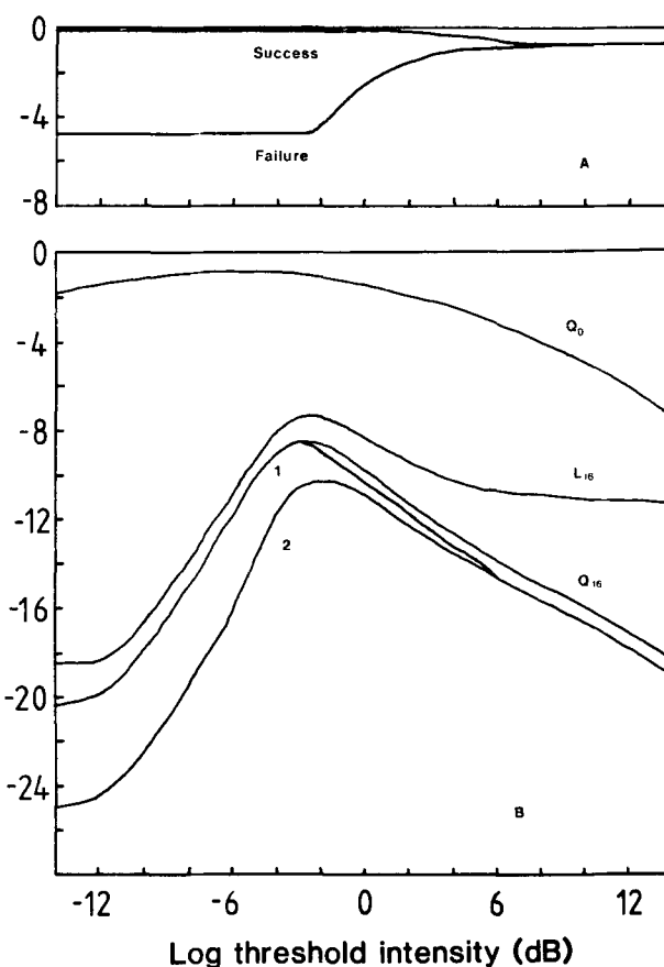
Figure 2. Construction of the quest function. The abscissa denotes possible values of T in steps of 1/20th of a \log_{10} unit (1 dB). Panel A shows the success and failure functions. In panel B, Q_0 is the quest function at trial 0, equal to the \log_{10} of the prior density. In this case, the prior density was specified as a normal distribution with a mean ( T_{\text{prior}} ) of -6 dB and a standard deviation of 8 dB. Curve Q_{16} is the quest function after trial 16. Curve L_{16} is the \log_{10} of the likelihood function of T following the 16th trial, and is equal to the difference between Q_0 and Q_{16} . The curve labeled 1 is the quest function after a successful trial 17 at an intensity of -3 dB. It is obtained by shifting the success function to the left by 3 dB and adding it to Q_{16} . Curve 2 is the quest function after a failure on trial 17, obtained by shifting and adding the failure function to Q_{16} .
