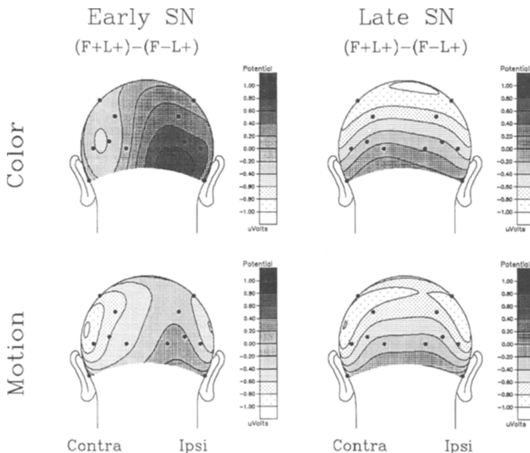
Figure 8. Isovoltage contour maps of the mean amplitude of the early (150–225 msec) and late (225–300 msec) SN in the [(F+L+)-(F-L+)] difference wave, which reflects feature selection at the attended location. As in Figure 5, maps are based on data averaged across left and right fields and hemispheres so that the hemisphere contralateral to the stimulus appears on the left side and the ipsilateral hemisphere on the right side. Note the change from an early contralateral to a later more symmetrical scalp distribution of the SN.
