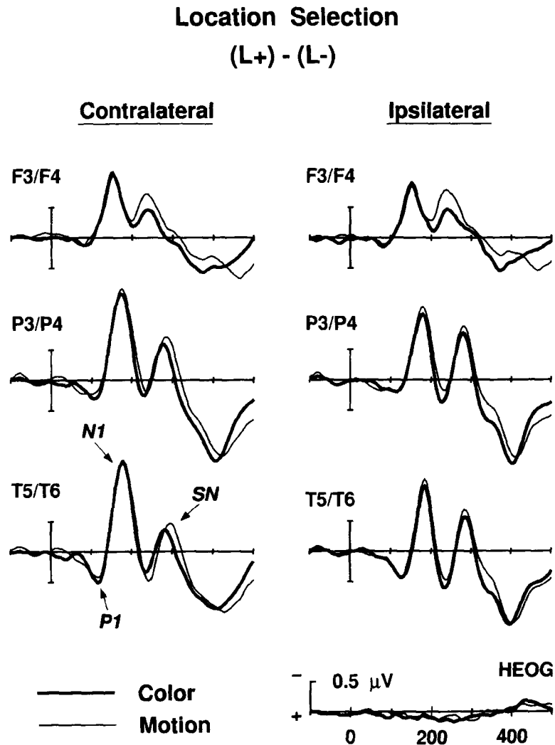
Figure 4. Difference waves obtained by subtracting grand-average ERPs to all standard stimuli presented in the unattended location (L-) from the ERPs to all standards presented in the attended location (L+). ERPs were averaged across stimuli with the attended feature value (F+) and without the attended feature (F-). Separate difference waves were calculated for the hemisphere contralateral (left column) and ipsilateral (right column) to the visual field of the stimulus. Superimposed traces correspond to the attend-color (thick line) and attend-motion (thin line) conditions.
