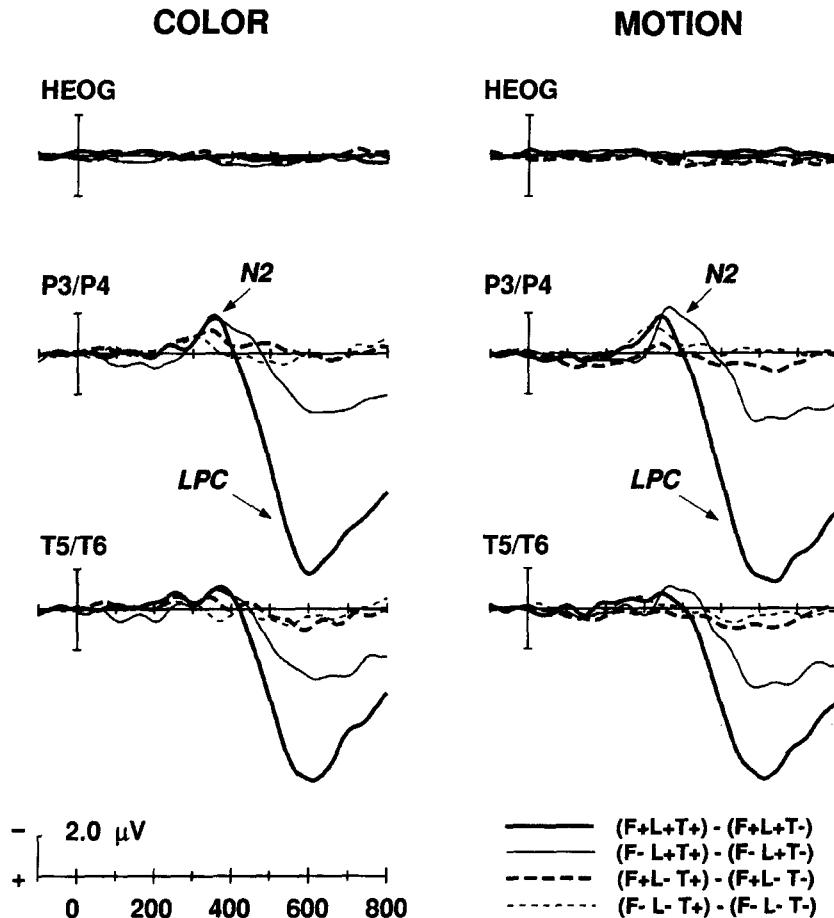
Figure 9. Difference waves obtained by subtracting grand-average ERPs to the standards ( T- ) from ERPs to the targets ( T+ ) for each of the four types of stimulus combinations indicated in the legend. Separate averages are shown for the attend-color (left column) and attend-motion (right column) conditions. ERPs shown are for the hemisphere contralateral to the visual field of stimulus presentation, collapsed over right and left hemisphere recordings.
