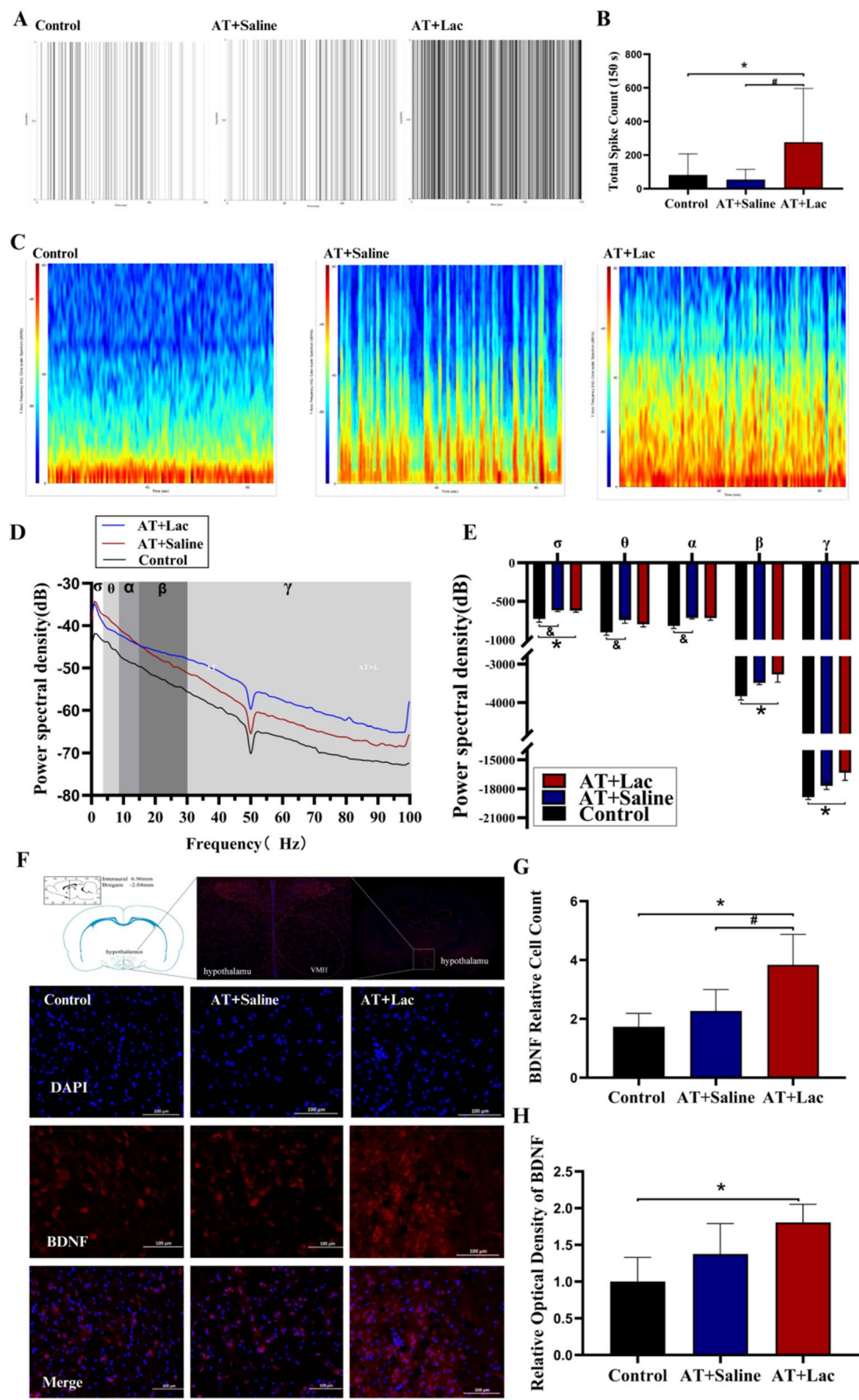
Fig. 7 LFPs, spike firing rate and BDNF expression of VMH in Exp. 2. A Spike firing point for 150 seconds; B Spike firing counts; C LFP spectrogram of the VMH for 3 minutes; D-E Power spectral density distribution and integration of \delta - \gamma bands; F IHC images of BDNF in the VMH (red: BDNF, blue: DAPI); G Number of BDNF positive cells; H Optical density of BDNF. *: AT+Lac vs Control, P < 0.05 ; #: AT+Lac vs AT-saline, P < 0.05 ; &: AT+Saline vs Control, P < 0.05
