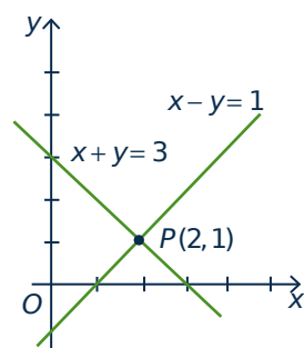
(a) Unique solution ( x = 2, y = 1 )
