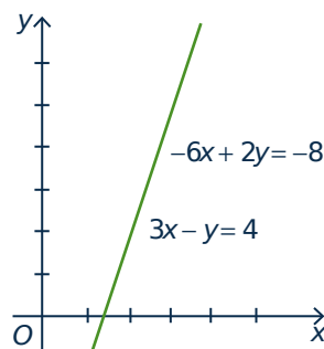
(c) Infinitely many solutions ( x = t, y = 3t - 4 )
