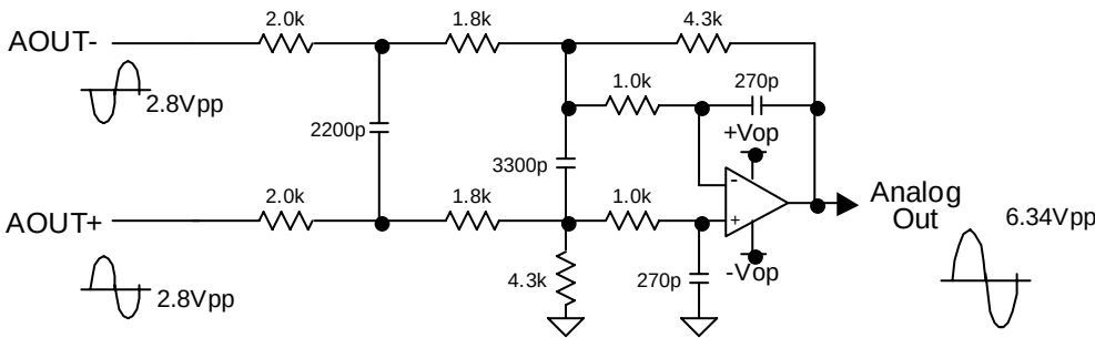
Figure 21. External 3rd Order LPF Circuit Example for DSD
