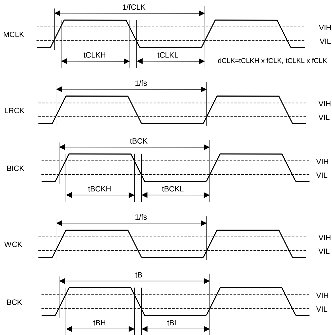
Clock Timing
