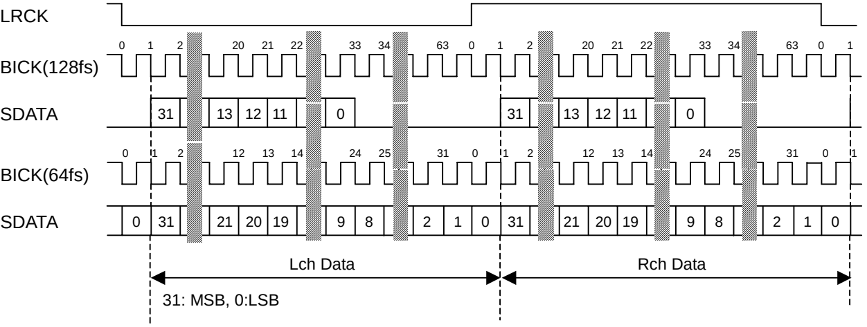
Figure 7. Mode 7 Timing
