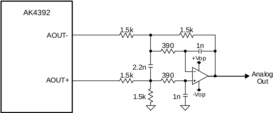
Figure 19. External LPF Circuit Example 1 for PCM (fc = 99.2kHz, Q=0.704)
