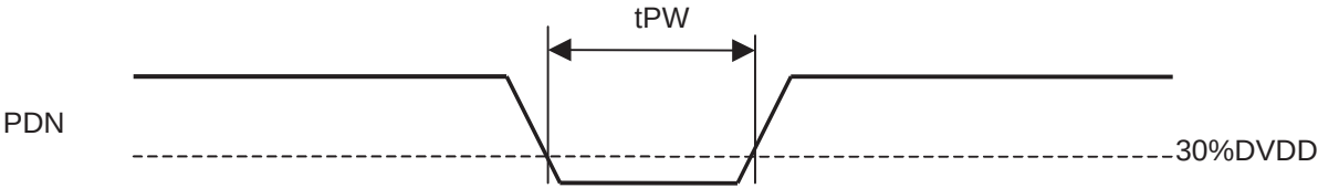
Power-down Timing
