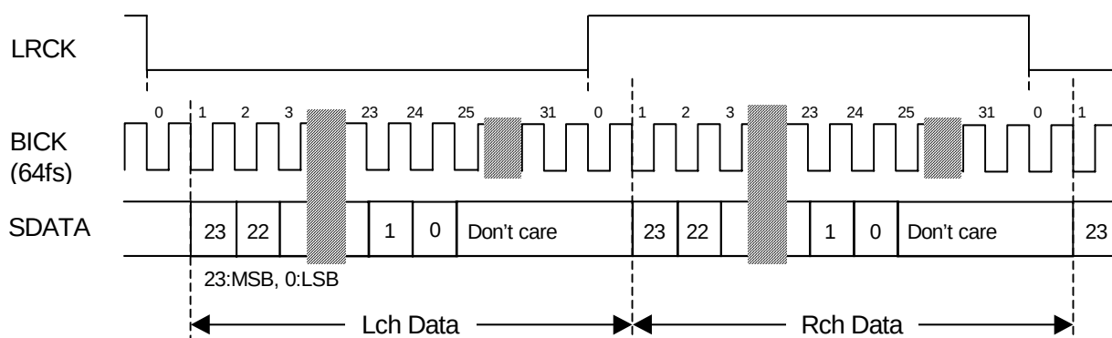
Figure 4. Mode 3 Timing
