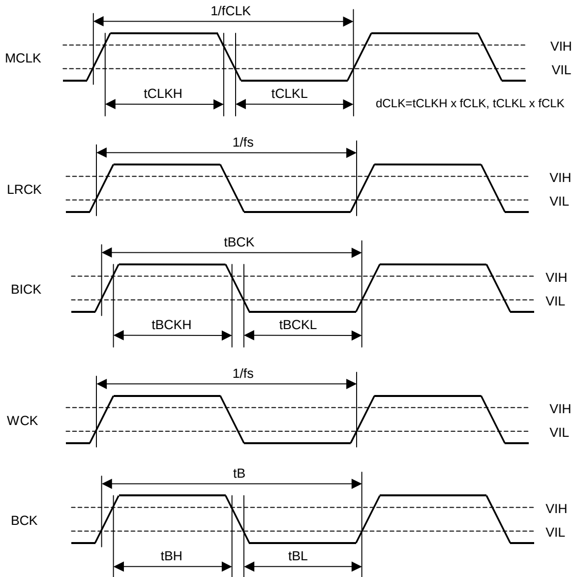
Clock Timing
