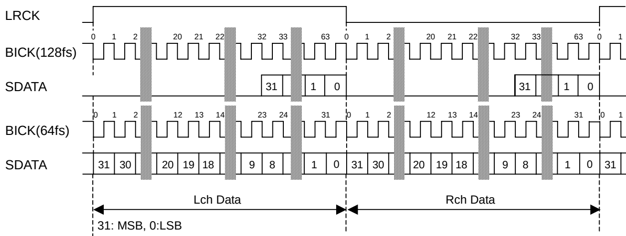
Figure 5. Mode 5 Timing
