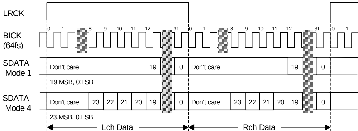
Figure 2. Mode 1/4 Timing
