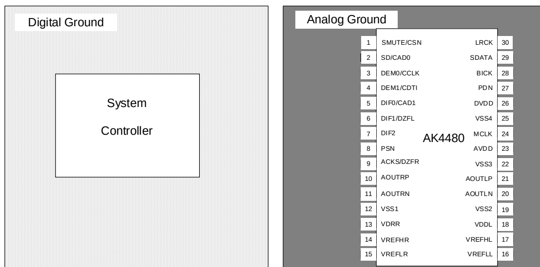
Figure 18. Ground Layout
