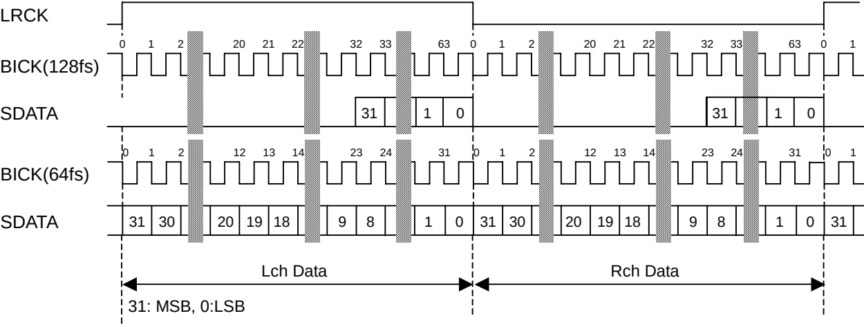
Figure 5. Mode 5 Timing
