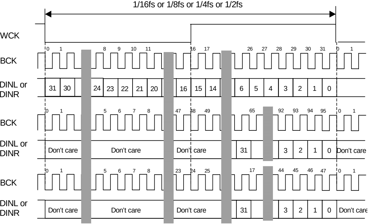
Figure 9. EX DF I/F Mode Timing
