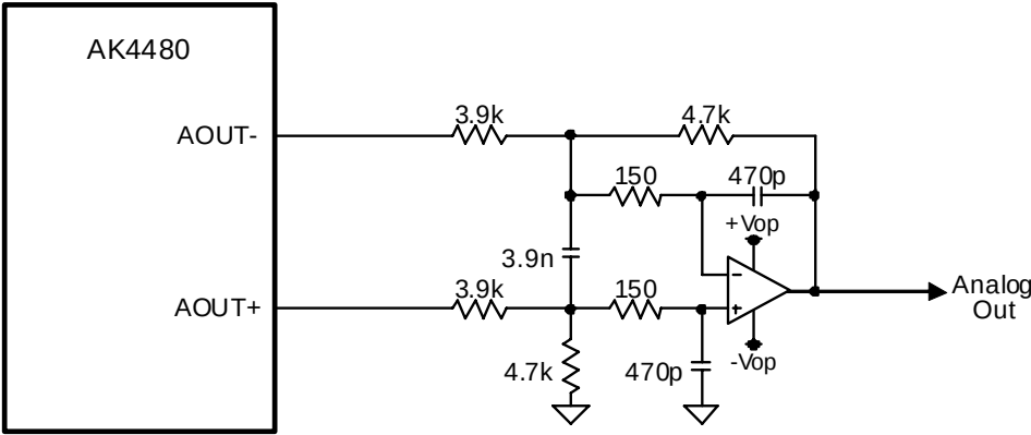
Figure 19. External LPF Circuit Example 1 for PCM (fc = 99.0kHz, Q=0.680)
