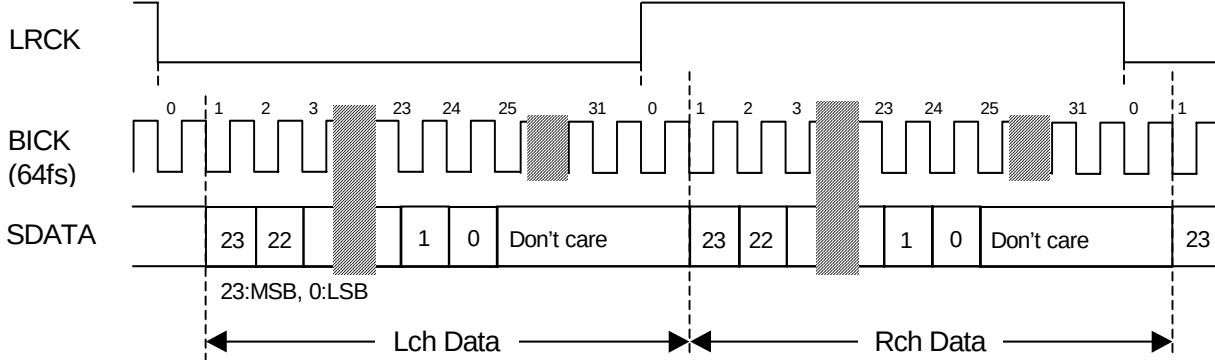
Figure 4. Mode 3 Timing
