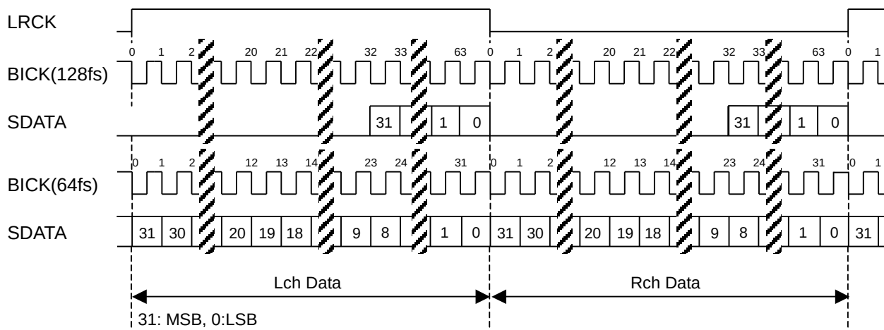
Figure 15. Mode 5 Timing
