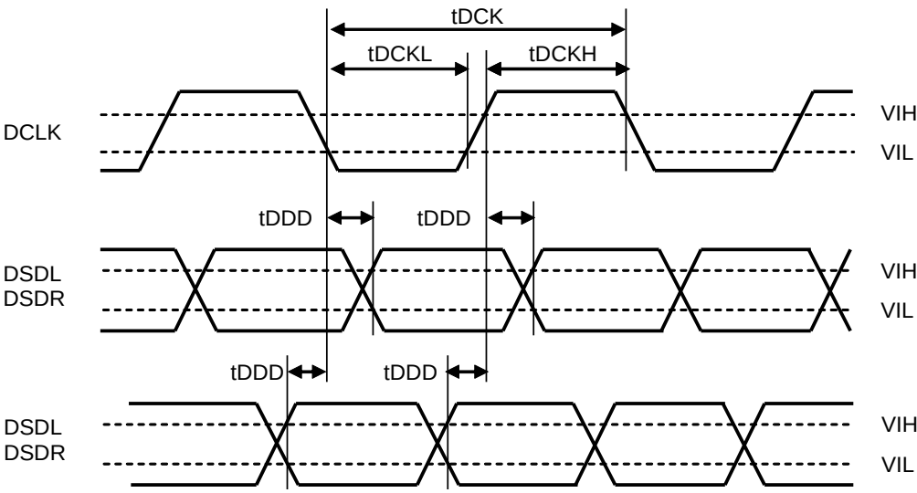
Audio Serial Interface Timing (DSD Phase Modulation Mode, DCKB bit = “0”)
