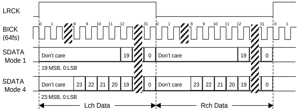
Figure 12. Mode 1/4 Timing
