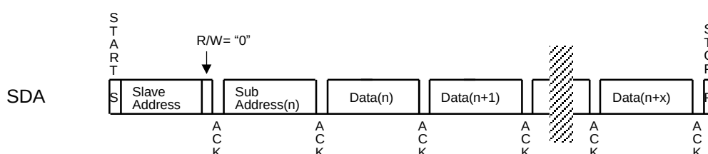
Figure 29. Data Transfer Sequence at I 2 C Bus Mode
