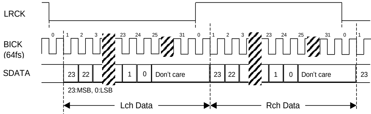
Figure 14. Mode 3 Timing
