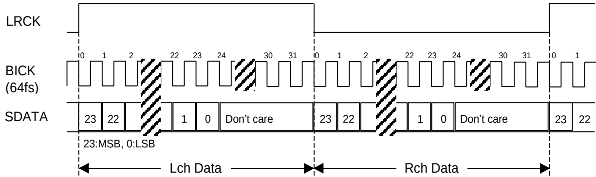
Figure 13. Mode 2 Timing
