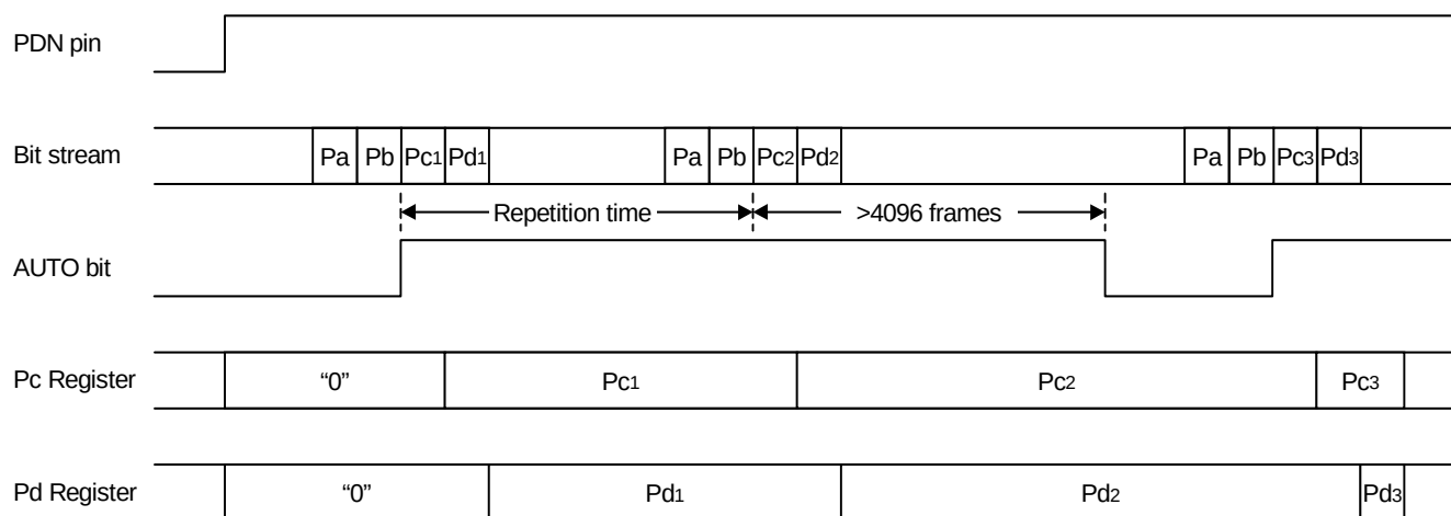
Figure 32. Timing example 1
