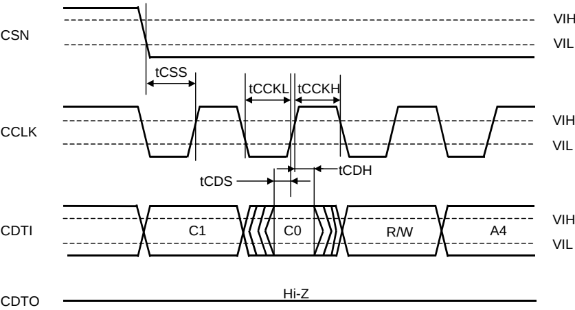
WRITE/READ Command Input Timing (4-wire serial mode)
