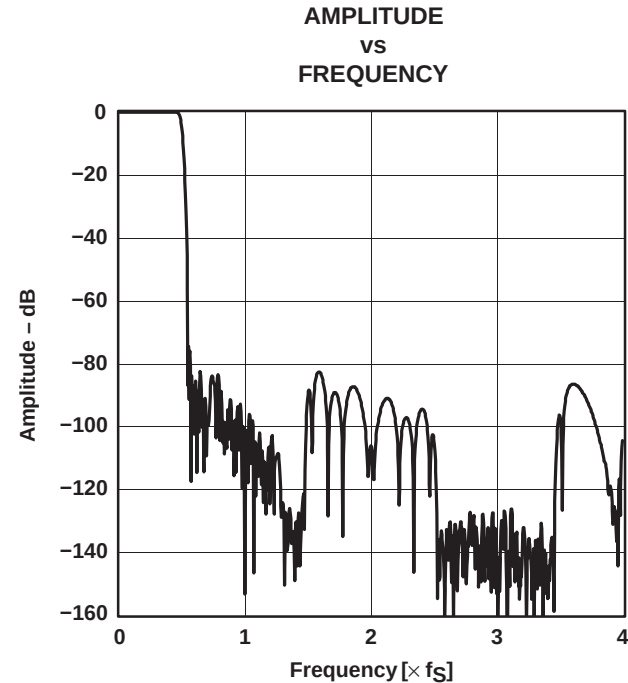
Figure 1. Frequency Response, Sharp Rolloff
