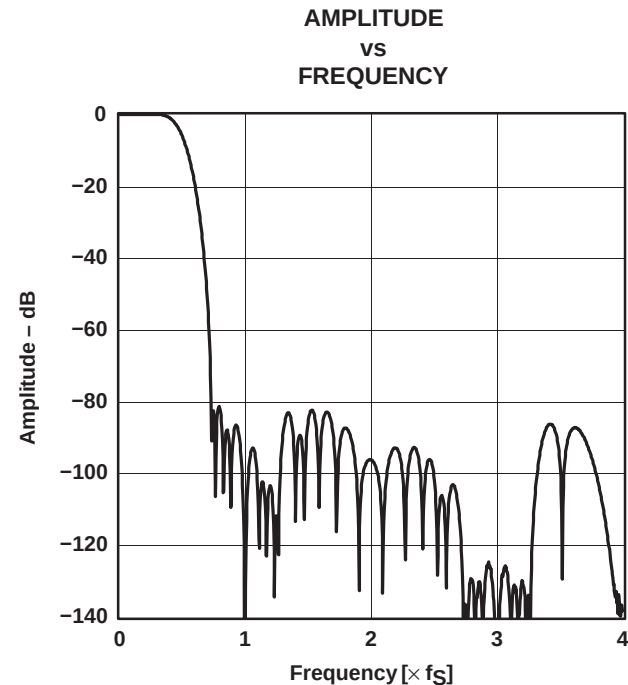
Figure 3. Frequency Response, Slow Rolloff
