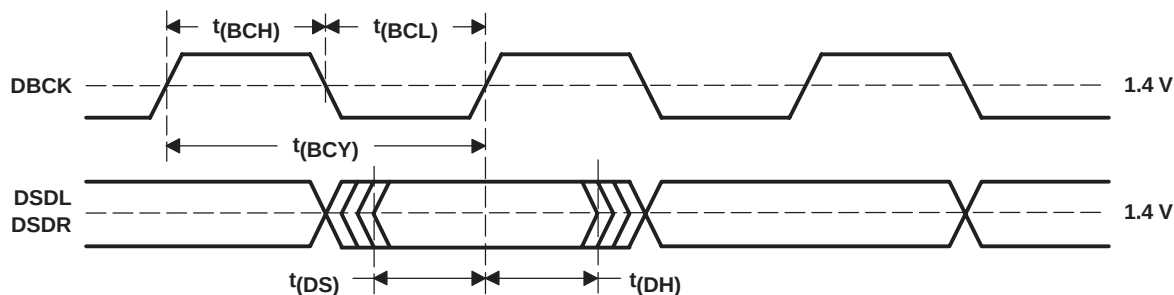
Figure 39. Normal Data Output Form From DSD Decoder
