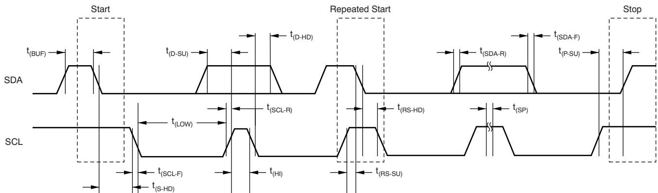
Figure 1. Timing Definition on the I²C Bus
