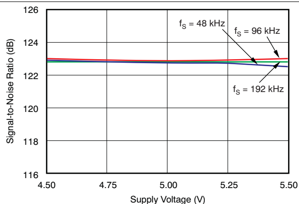
Figure 14. SNR vs Supply Voltage
