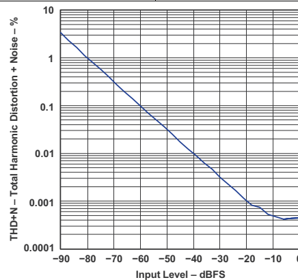
Figure 25. Total Harmonic Distortion + Noise vs Input Level
