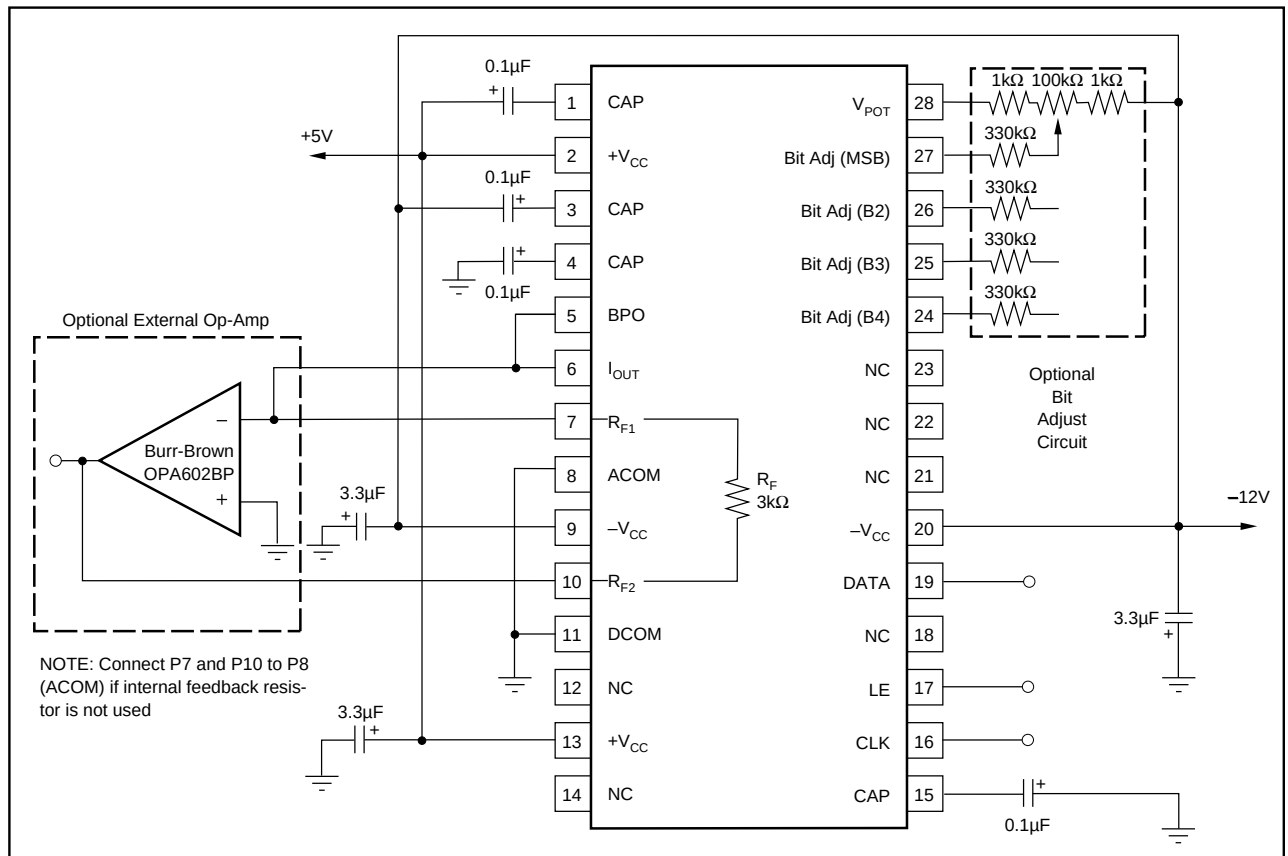
FIGURE 4. PCM58P Connection Diagram.
