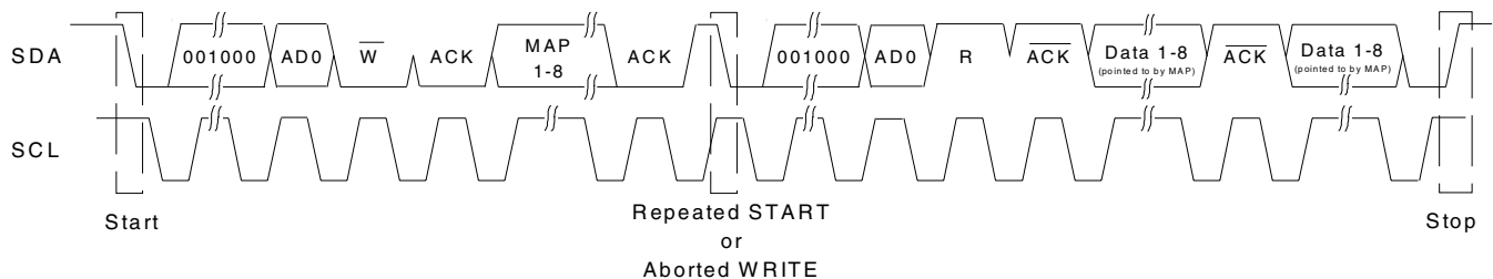
Figure 20. I²C Read
