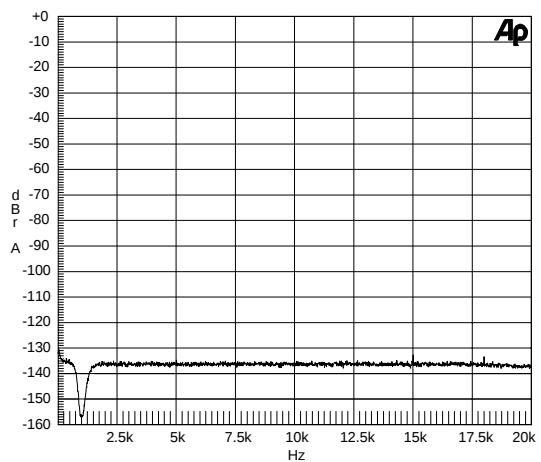
Figure 17. -20 dBFS FFT
