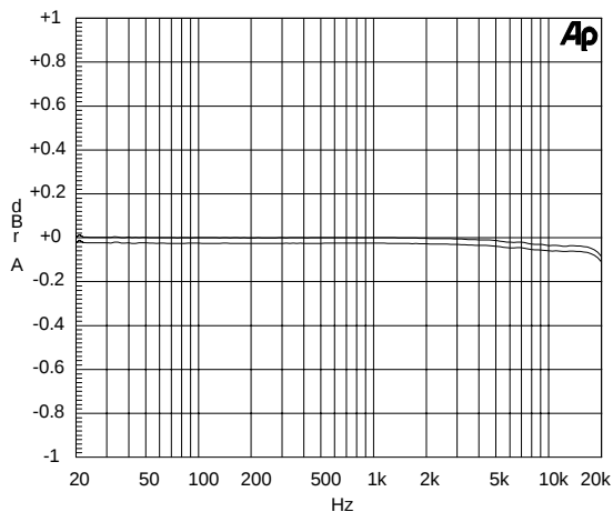
Figure 14. Frequency Response
