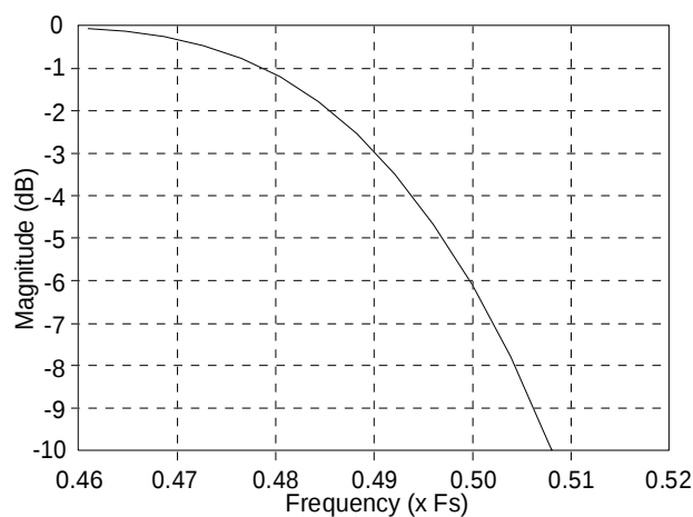
Figure 11. Combined Digital and Analog Filter
