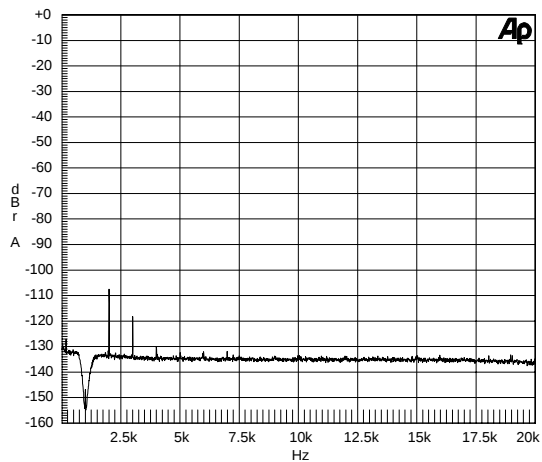
Figure 16. 0 dBFS FFT
