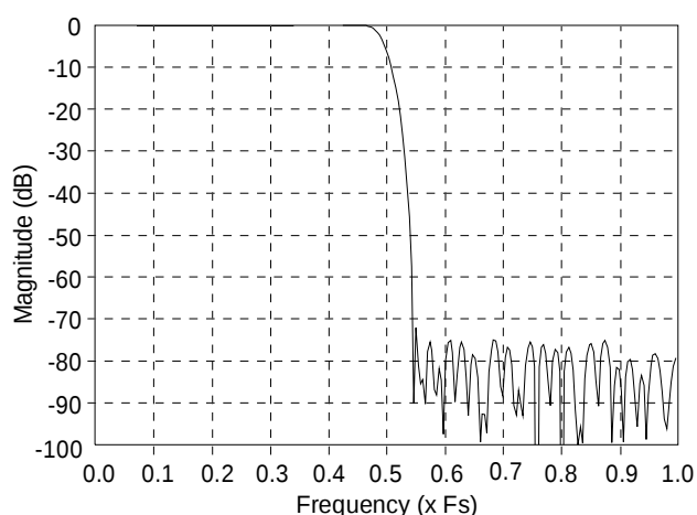
Figure 9. CS4390 Combined Digital and Analog Filter Stopband Rejection
