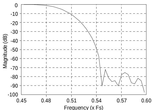
Figure 10. CS4390 Combined Digital and Analog Filter
