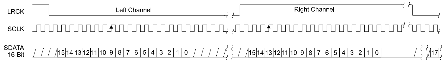
Figure 6. Digital Input Format 5.
