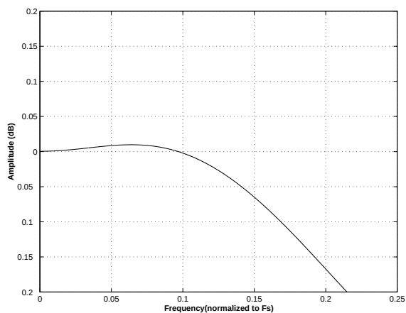
Figure 31. Quad Speed (fast) Passband Ripple
