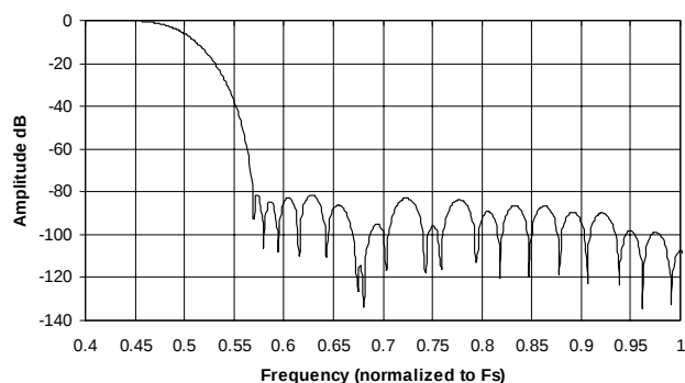
Figure 13. Double-speed Stopband
