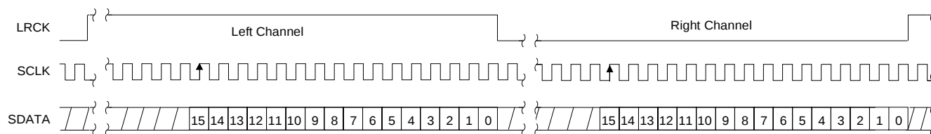
Figure 31. Format 2, Right Justified, 16-Bit Data
