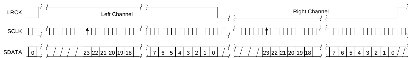
Figure 32. Format 3, Right Justified, 24-Bit Data
