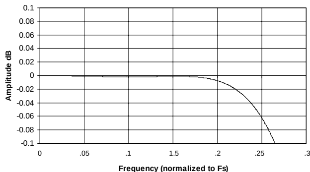
Figure 24. 8x Interpolator Frequency Response
