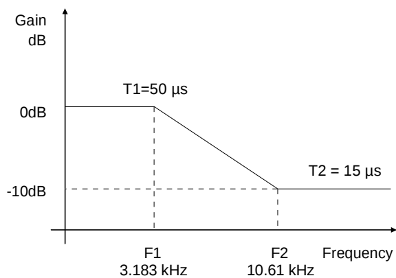
Figure 28. De-Emphasis Curve
