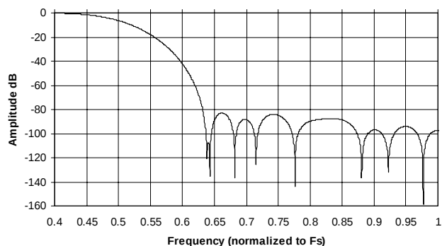
Figure 17. Quad-speed Stopband Rejection
