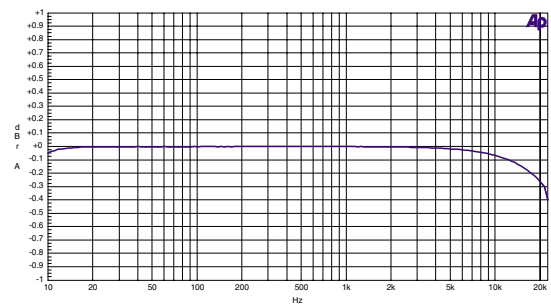
Figure 29. Frequency response
