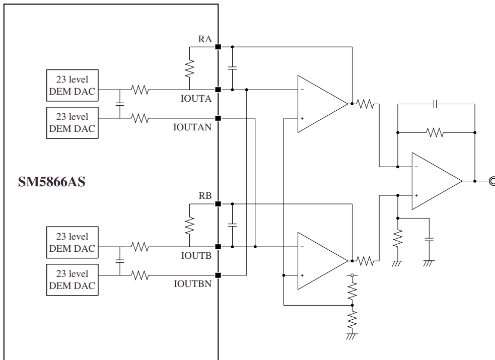
Figure 14. Connection example 1
