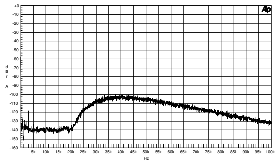
Figure 17. 0dB input FFT (with 1kHz notch filter 32768 pts. 8 average)
