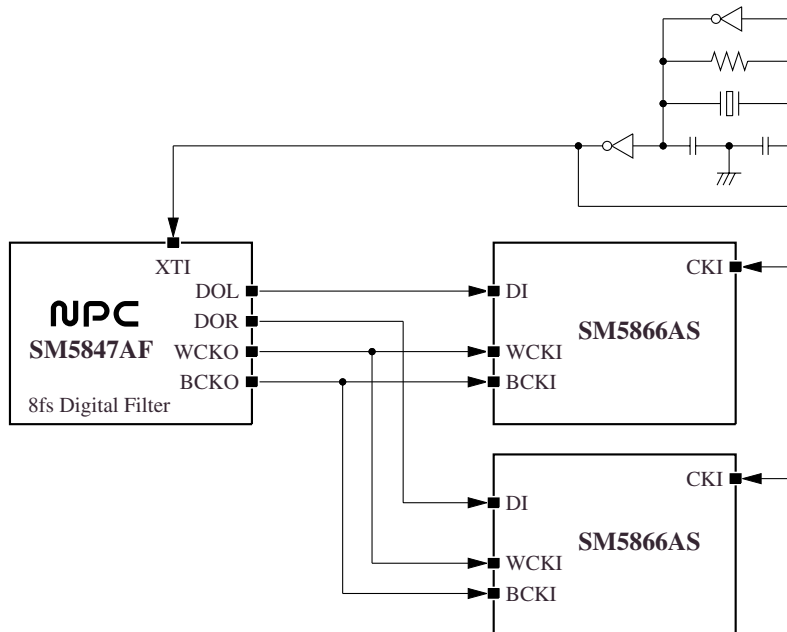
Figure 13. PCM Mode input interface connection example
