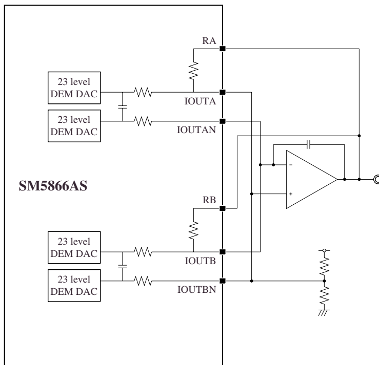
Figure 15. Connection example 2
